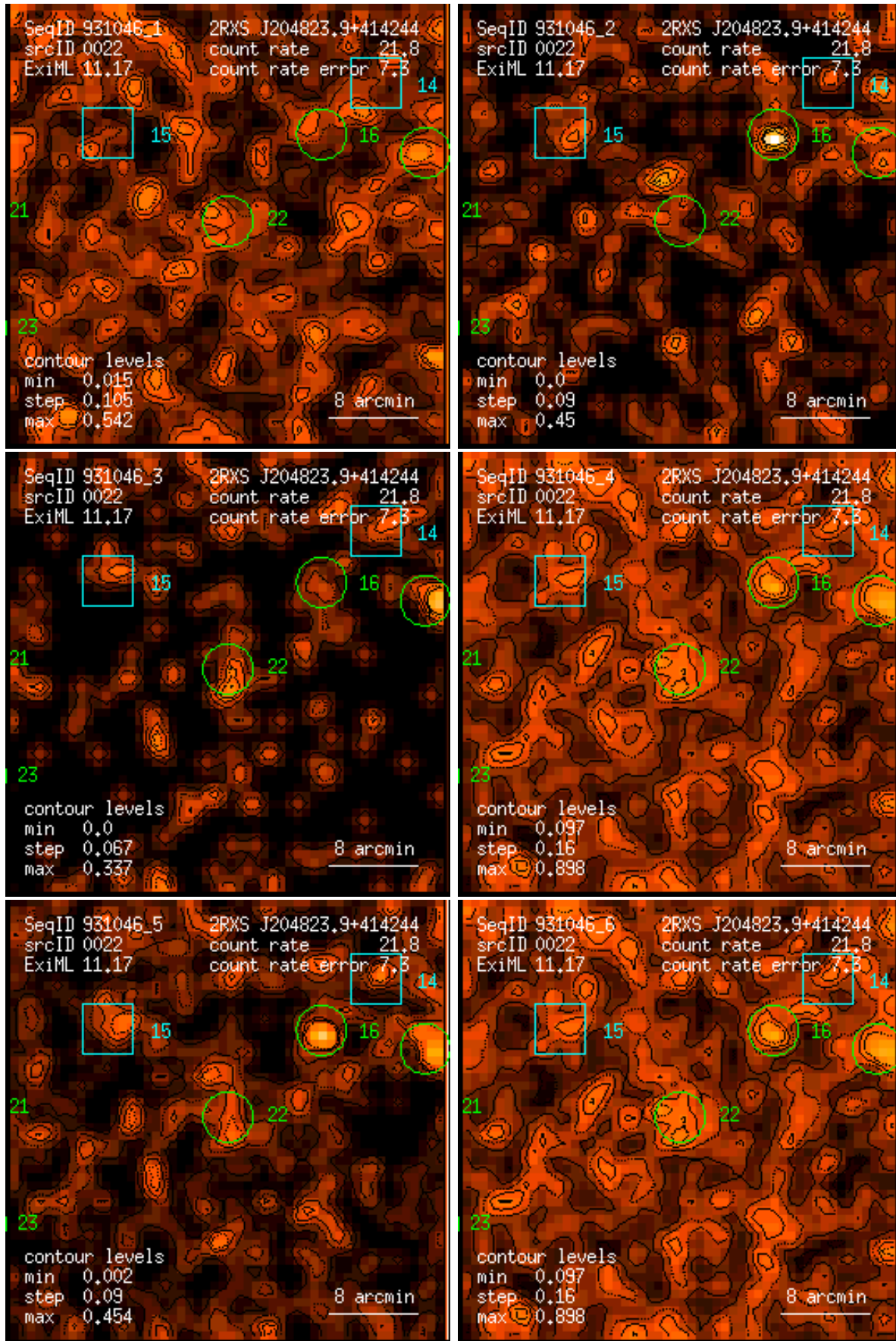
Figure 22: RASS 931046: detection 0022: band rate images, Gaussian filter: (1) PSPC channels 11 – 41, (2) 52 – 90, (3) 91 – 201, (4) 11 – 235, (5) 52 – 201, (6) 11 – 201. Broad band rates in counts/ks. Band rate contour levels in counts/ks/arcmin 2 .
