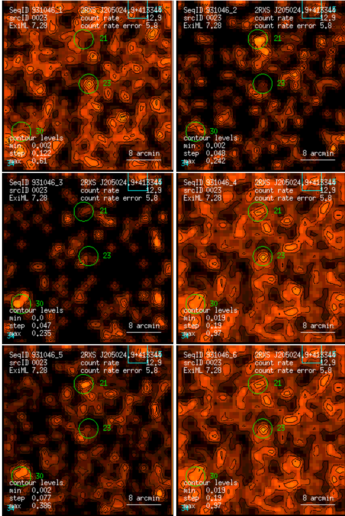
Figure 23: RASS 931046: detection 0023: band rate images, Gaussian filter: (1) PSPC channels 11 – 41, (2) 52 – 90, (3) 91 – 201, (4) 11 – 235, (5) 52 – 201, (6) 11 – 201. Broad band rates in counts/ks. Band rate contour levels in counts/ks/arcmin 2 .
