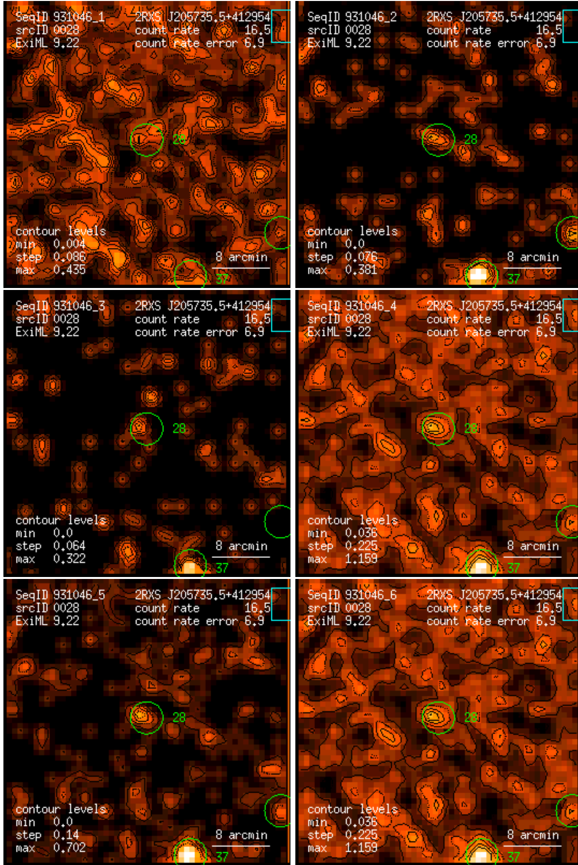
Figure 28: RASS 931046: detection 0028: band rate images, Gaussian filter: (1) PSPC channels 11 – 41, (2) 52 – 90, (3) 91 – 201, (4) 11 – 235, (5) 52 – 201, (6) 11 – 201. Broad band rates in counts/ks. Band rate contour levels in counts/ks/arcmin 2 .
