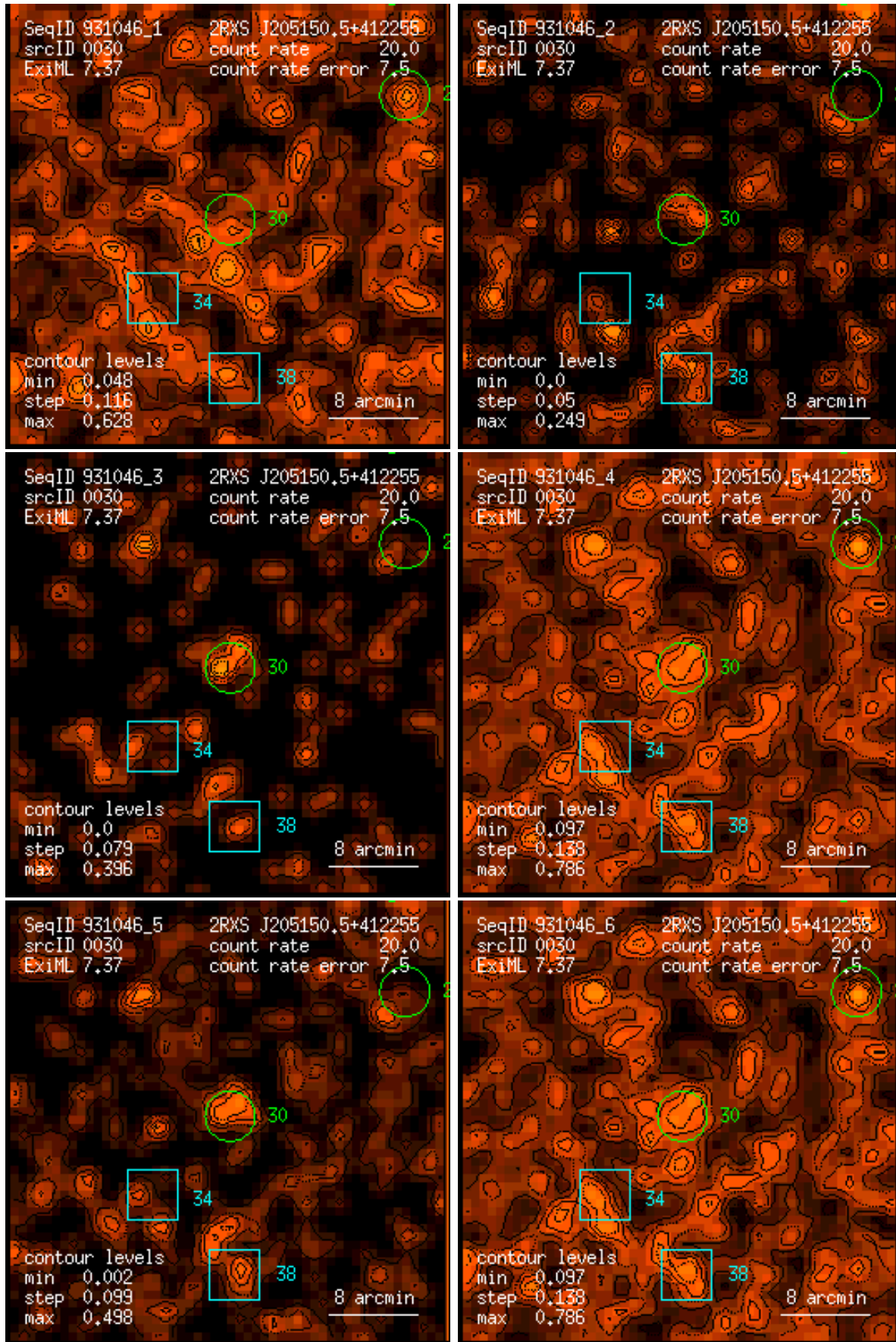
Figure 30: RASS 931046: detection 0030: band rate images, Gaussian filter: (1) PSPC channels 11 – 41, (2) 52 – 90, (3) 91 – 201, (4) 11 – 235, (5) 52 – 201, (6) 11 – 201. Broad band rates in counts/ks. Band rate contour levels in counts/ks/arcmin 2 .
