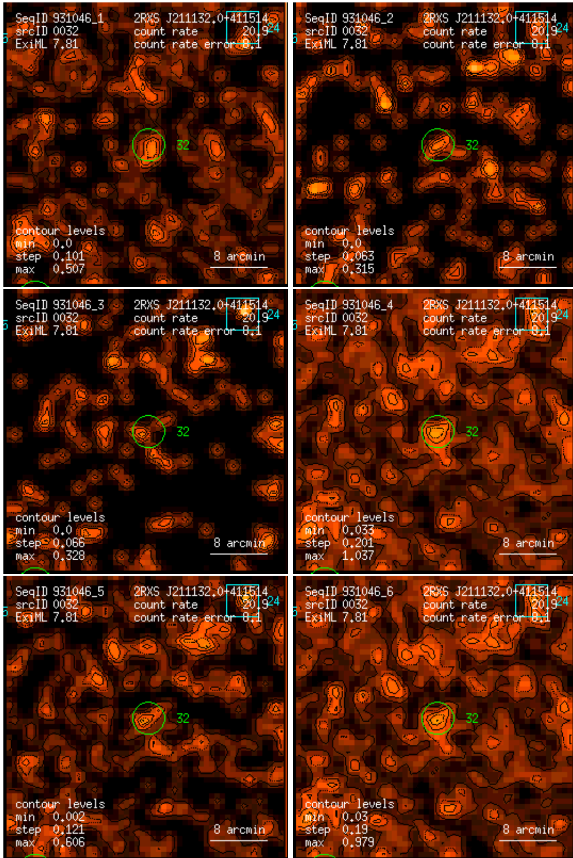
Figure 32: RASS 931046: detection 0032: band rate images, Gaussian filter: (1) PSPC channels 11 – 41, (2) 52 – 90, (3) 91 – 201, (4) 11 – 235, (5) 52 – 201, (6) 11 – 201. Broad band rates in counts/ks. Band rate contour levels in counts/ks/arcmin 2 .
