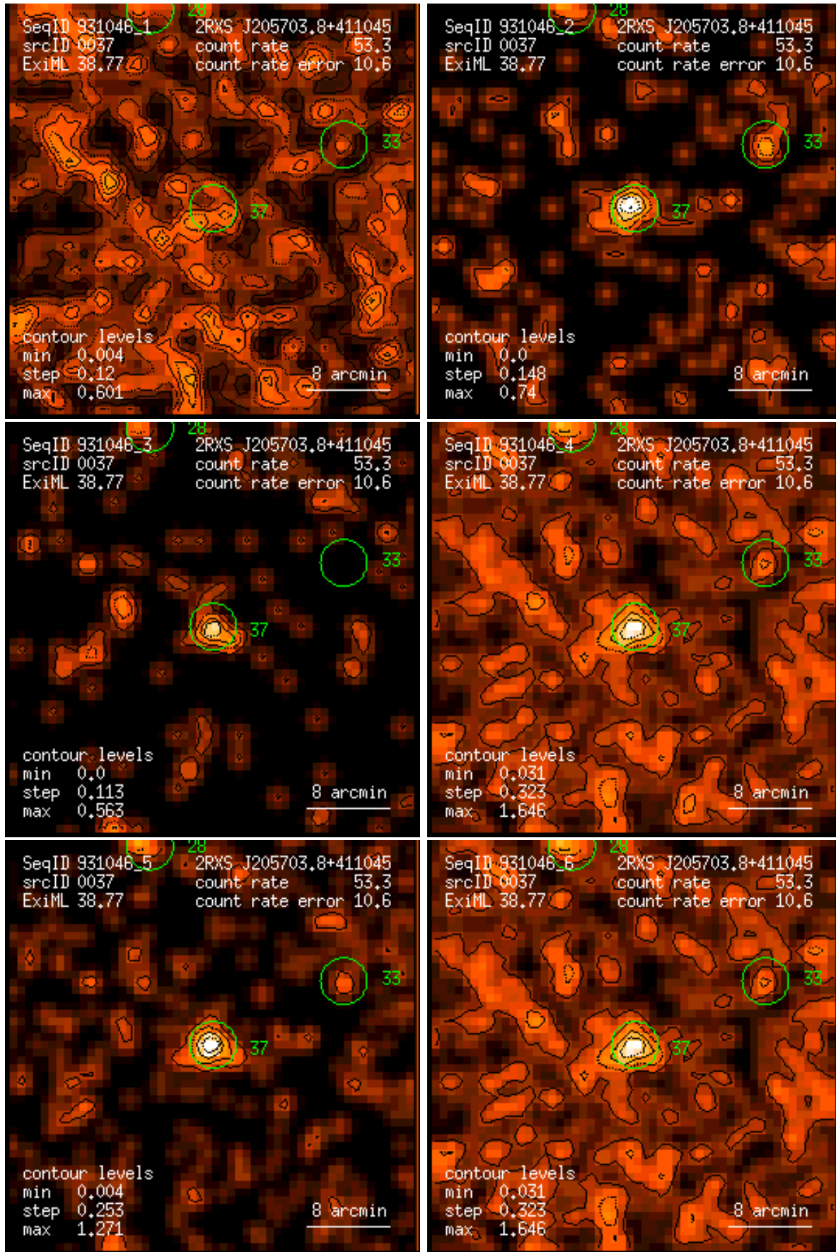
Figure 37: RASS 931046: detection 0037: band rate images, Gaussian filter: (1) PSPC channels 11 – 41, (2) 52 – 90, (3) 91 – 201, (4) 11 – 235, (5) 52 – 201, (6) 11 – 201. Broad band rates in counts/ks. Band rate contour levels in counts/ks/arcmin 2 .
