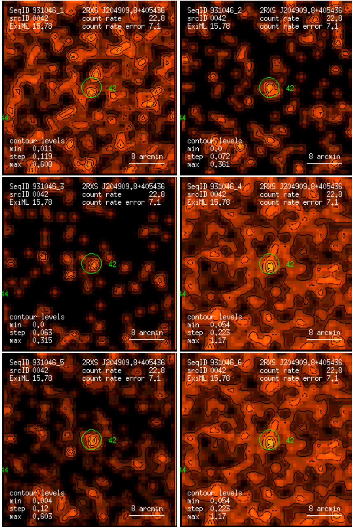
Figure 42: RASS 931046: detection 0042: band rate images, Gaussian filter: (1) PSPC channels 11 – 41, (2) 52 – 90, (3) 91 – 201, (4) 11 – 235, (5) 52 – 201, (6) 11 – 201. Broad band rates in counts/ks. Band rate contour levels in counts/ks/arcmin 2 .
