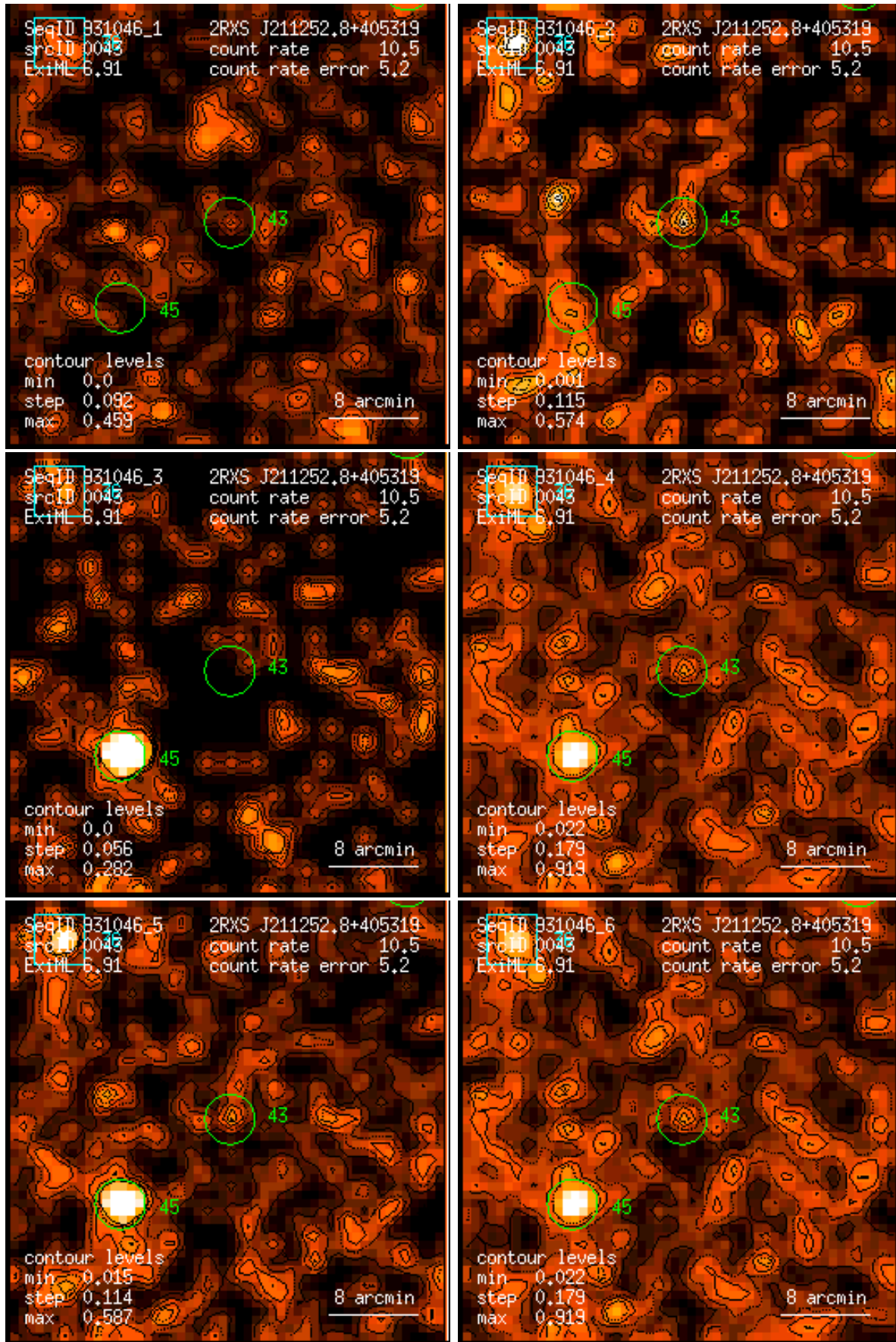
Figure 43: RASS 931046: detection 0043: band rate images, Gaussian filter: (1) PSPC channels 11 – 41, (2) 52 – 90, (3) 91 – 201, (4) 11 – 235, (5) 52 – 201, (6) 11 – 201. Broad band rates in counts/ks. Band rate contour levels in counts/ks/arcmin 2 .
