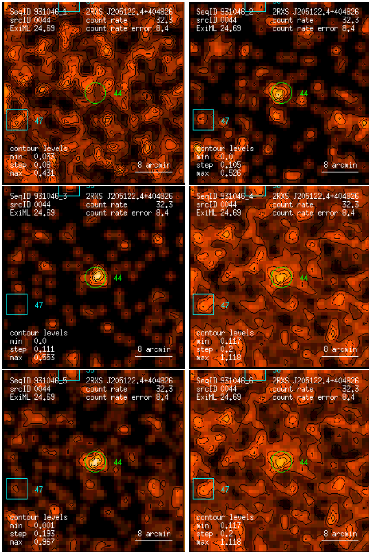
Figure 44: RASS 931046: detection 0044: band rate images, Gaussian filter: (1) PSPC channels 11 – 41, (2) 52 – 90, (3) 91 – 201, (4) 11 – 235, (5) 52 – 201, (6) 11 – 201. Broad band rates in counts/ks. Band rate contour levels in counts/ks/arcmin 2 .
