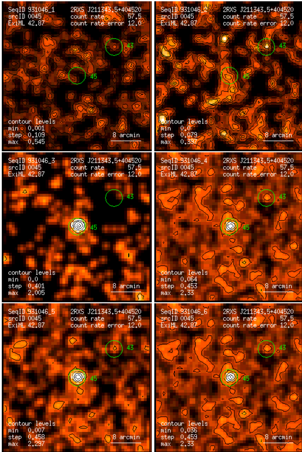
Figure 45: RASS 931046: detection 0045: band rate images, Gaussian filter: (1) PSPC channels 11 – 41, (2) 52 – 90, (3) 91 – 201, (4) 11 – 235, (5) 52 – 201, (6) 11 – 201. Broad band rates in counts/ks. Band rate contour levels in counts/ks/arcmin 2 .
