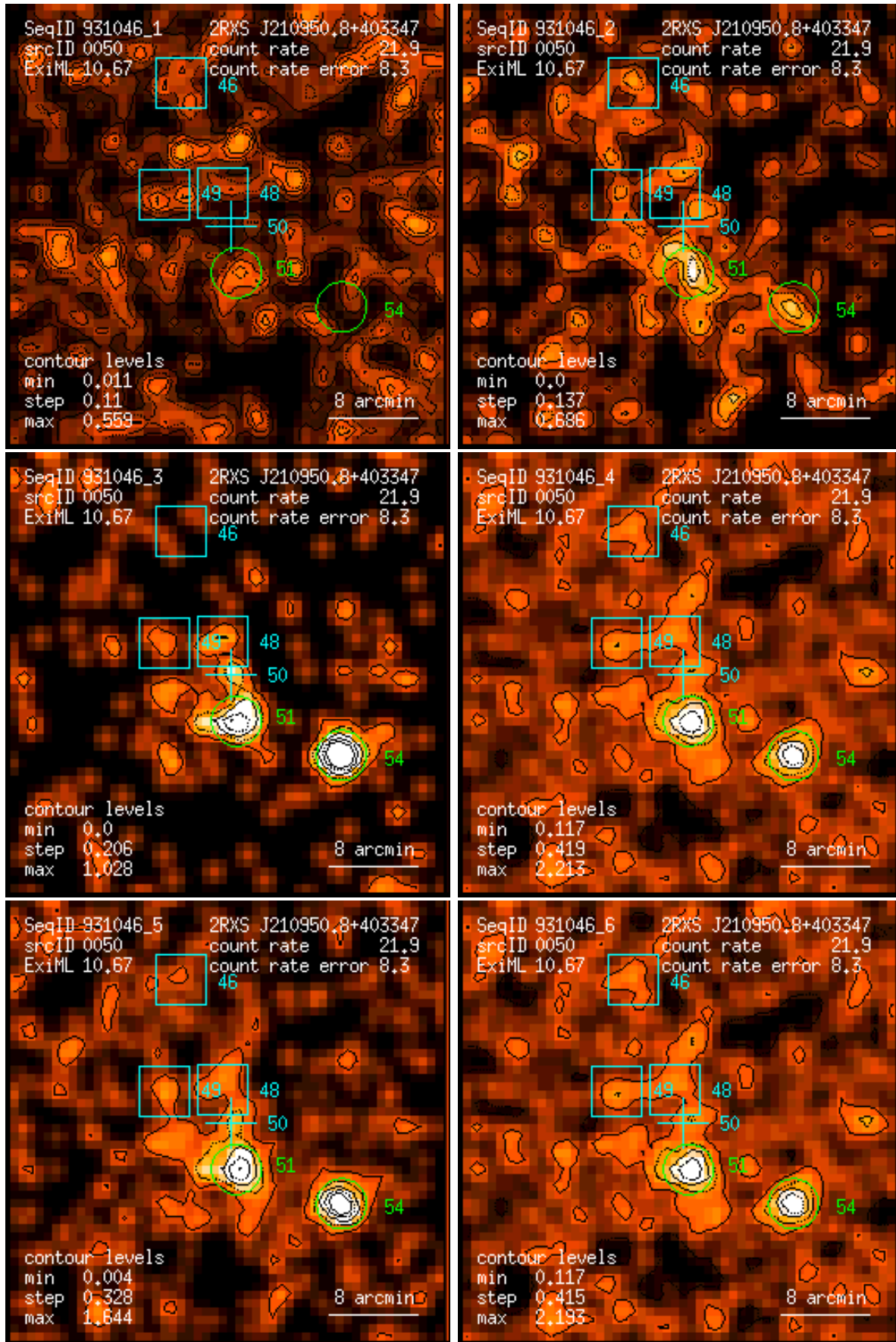
Figure 50: RASS 931046: detection 0050: band rate images, Gaussian filter: (1) PSPC channels 11 – 41, (2) 52 – 90, (3) 91 – 201, (4) 11 – 235, (5) 52 – 201, (6) 11 – 201. Broad band rates in counts/ks. Band rate contour levels in counts/ks/arcmin 2 .
