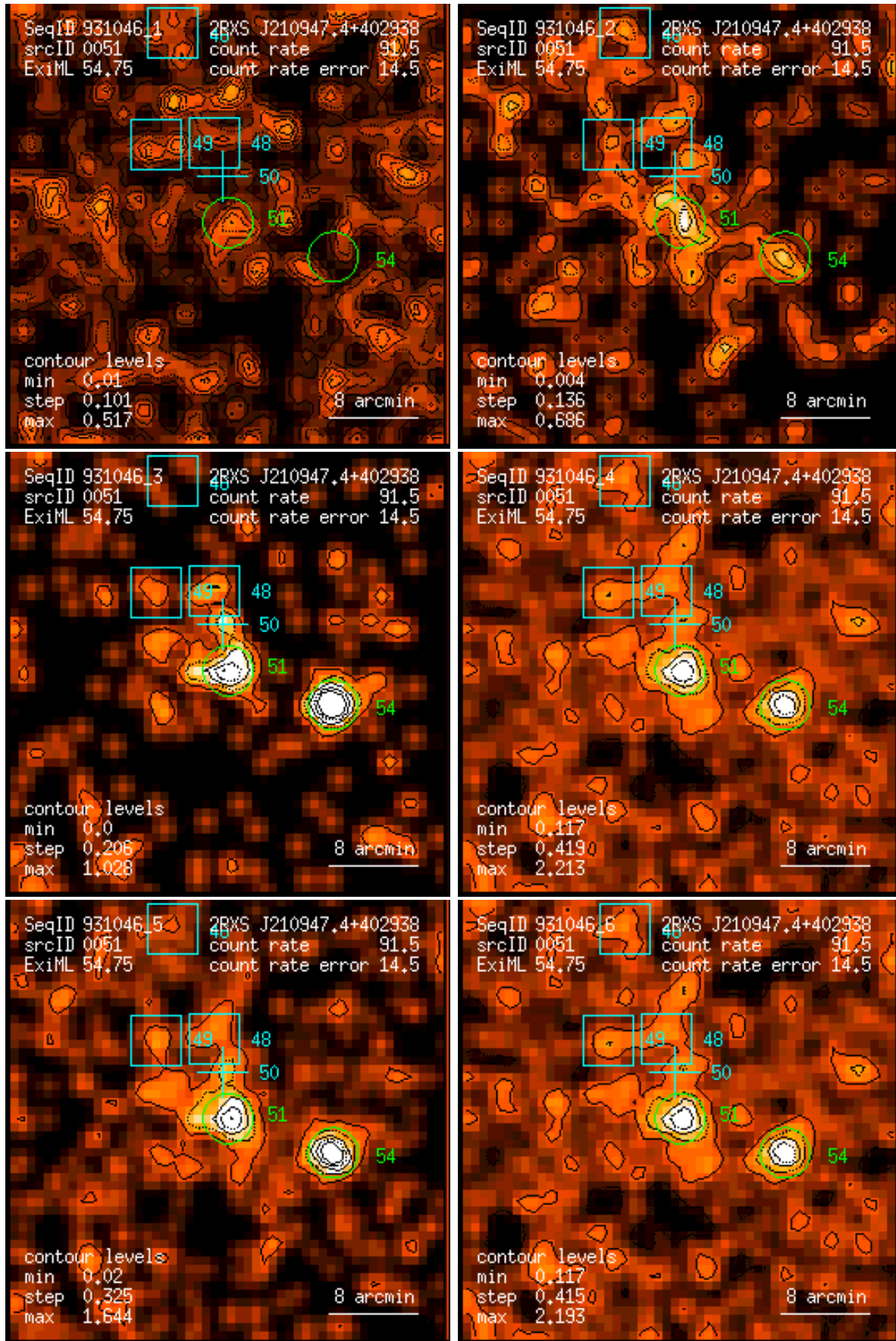
Figure 51: RASS 931046: detection 0051: band rate images, Gaussian filter: (1) PSPC channels 11 – 41, (2) 52 – 90, (3) 91 – 201, (4) 11 – 235, (5) 52 – 201, (6) 11 – 201. Broad band rates in counts/ks. Band rate contour levels in counts/ks/arcmin 2 .
