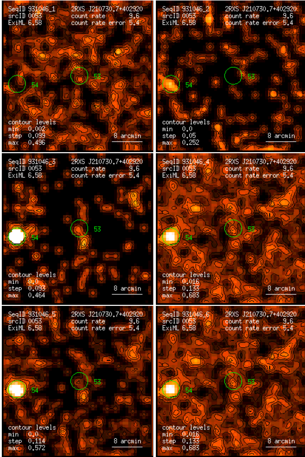
Figure 53: RASS 931046: detection 0053: band rate images, Gaussian filter: (1) PSPC channels 11 – 41, (2) 52 – 90, (3) 91 – 201, (4) 11 – 235, (5) 52 – 201, (6) 11 – 201. Broad band rates in counts/ks. Band rate contour levels in counts/ks/arcmin 2 .
