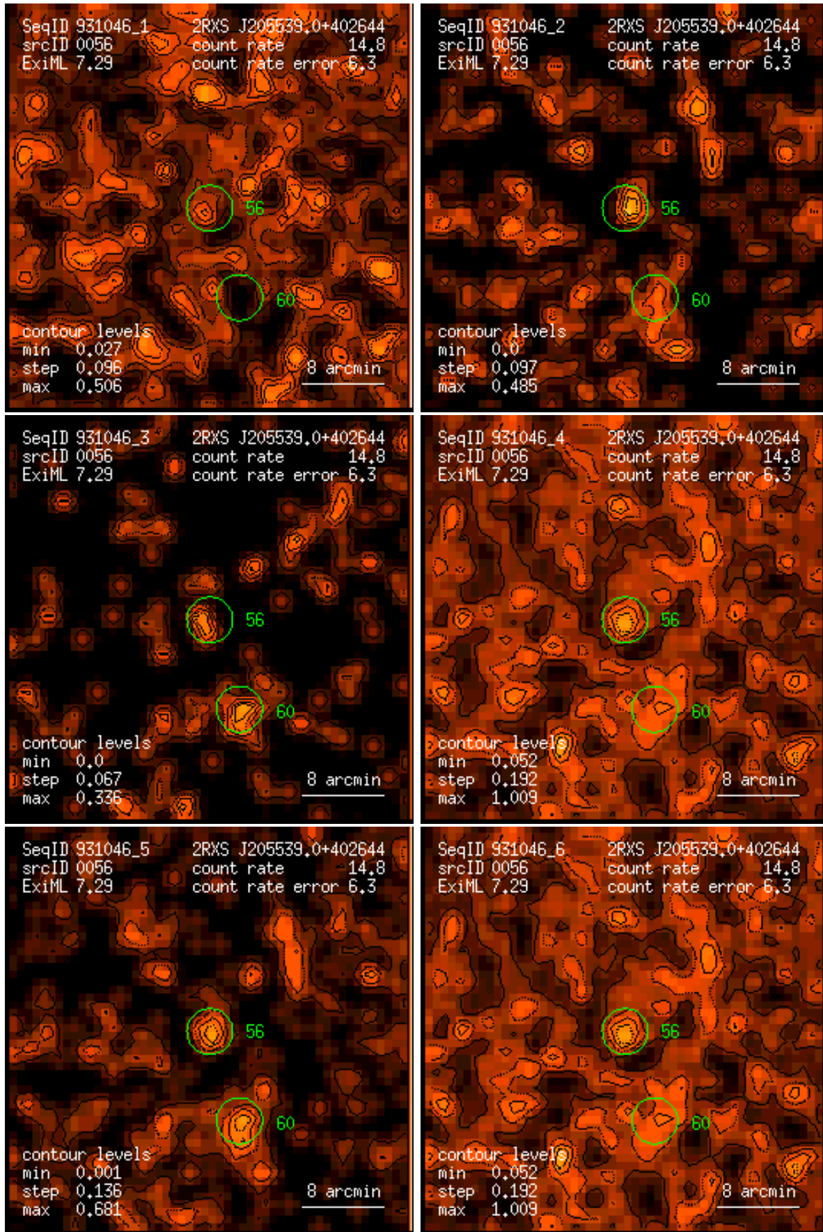
Figure 56: RASS 931046: detection 0056: band rate images, Gaussian filter: (1) PSPC channels 11 – 41, (2) 52 – 90, (3) 91 – 201, (4) 11 – 235, (5) 52 – 201, (6) 11 – 201. Broad band rates in counts/ks. Band rate contour levels in counts/ks/arcmin 2 .
