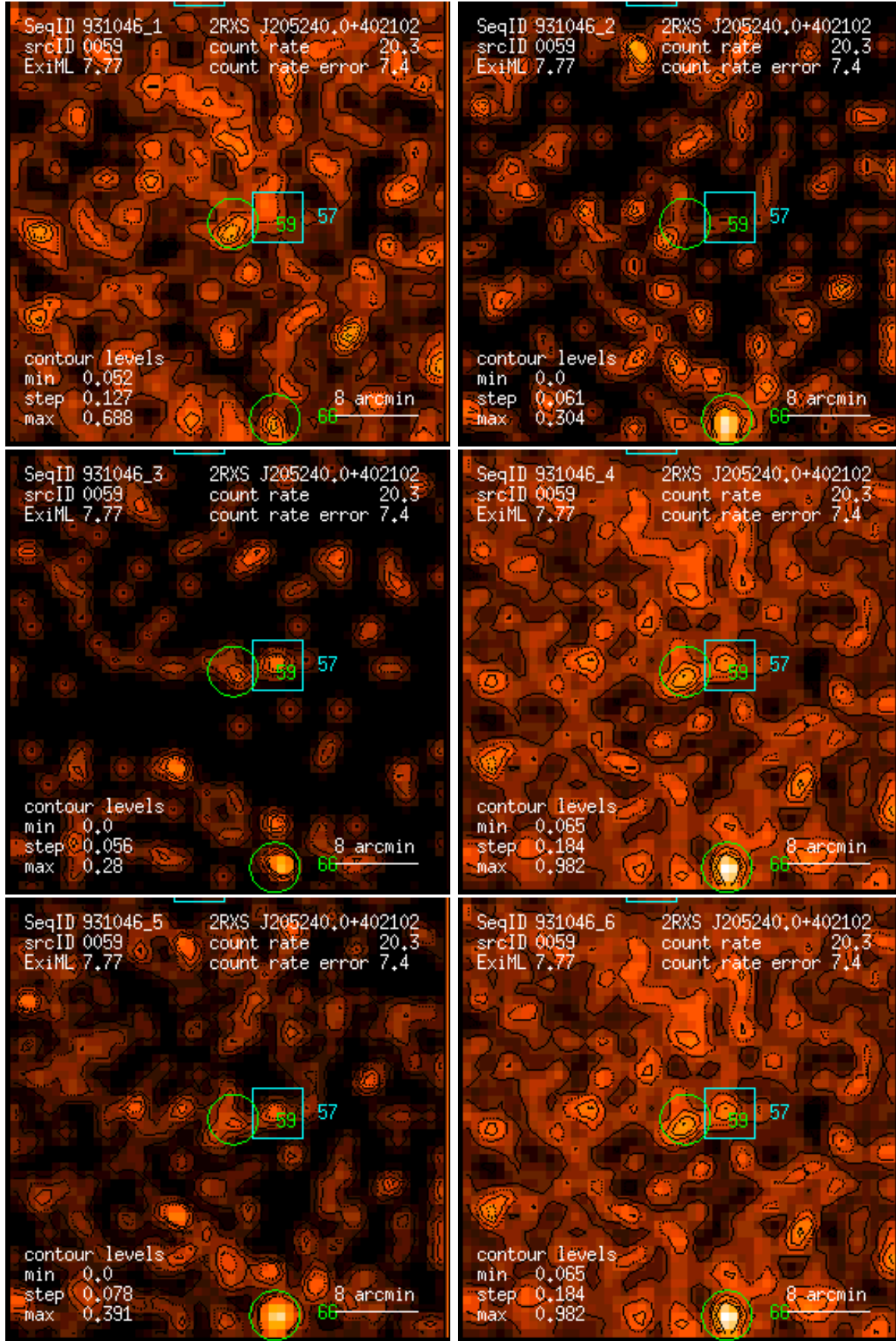
Figure 59: RASS 931046: detection 0059: band rate images, Gaussian filter: (1) PSPC channels 11 – 41, (2) 52 – 90, (3) 91 – 201, (4) 11 – 235, (5) 52 – 201, (6) 11 – 201. Broad band rates in counts/ks. Band rate contour levels in counts/ks/arcmin 2 .
