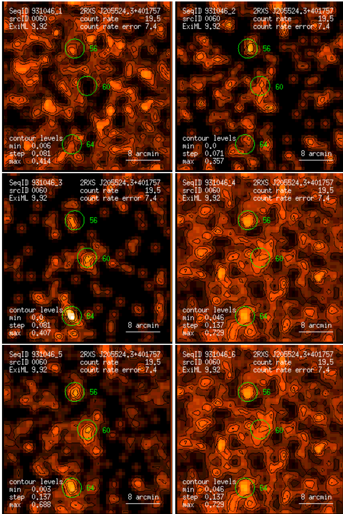
Figure 60: RASS 931046: detection 0060: band rate images, Gaussian filter: (1) PSPC channels 11 – 41, (2) 52 – 90, (3) 91 – 201, (4) 11 – 235, (5) 52 – 201, (6) 11 – 201. Broad band rates in counts/ks. Band rate contour levels in counts/ks/arcmin 2 .
