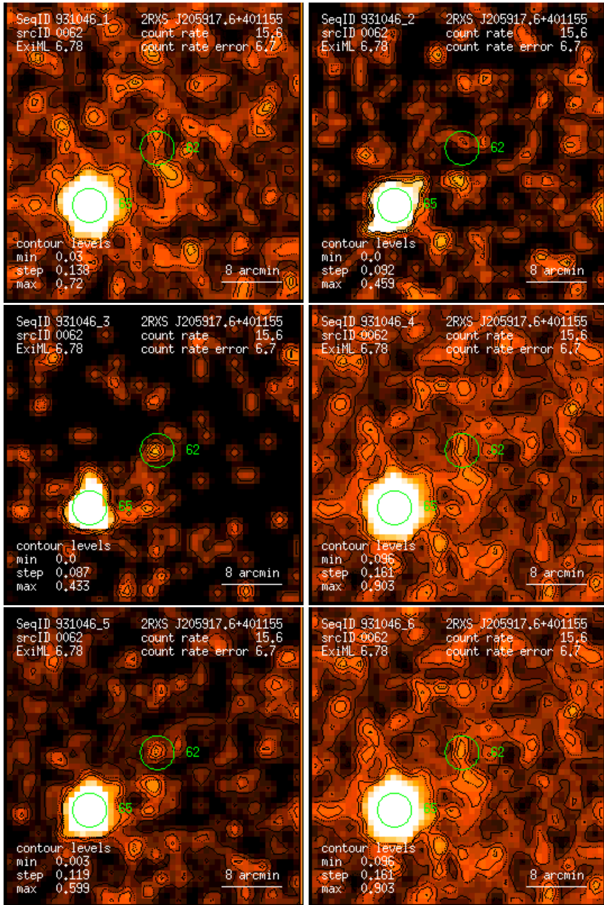
Figure 62: RASS 931046: detection 0062: band rate images, Gaussian filter: (1) PSPC channels 11 – 41, (2) 52 – 90, (3) 91 – 201, (4) 11 – 235, (5) 52 – 201, (6) 11 – 201. Broad band rates in counts/ks. Band rate contour levels in counts/ks/arcmin 2 .
