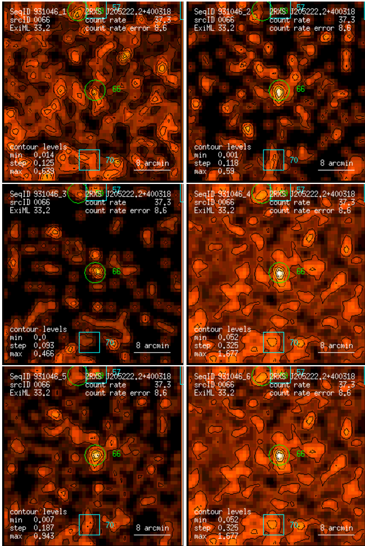
Figure 66: RASS 931046: detection 0066: band rate images, Gaussian filter: (1) PSPC channels 11 – 41, (2) 52 – 90, (3) 91 – 201, (4) 11 – 235, (5) 52 – 201, (6) 11 – 201. Broad band rates in counts/ks. Band rate contour levels in counts/ks/arcmin 2 .
