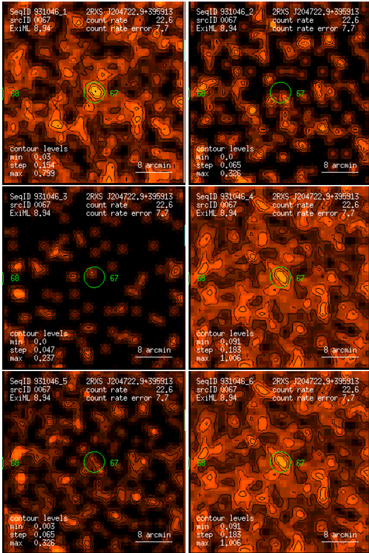
Figure 67: RASS 931046: detection 0067: band rate images, Gaussian filter: (1) PSPC channels 11 – 41, (2) 52 – 90, (3) 91 – 201, (4) 11 – 235, (5) 52 – 201, (6) 11 – 201. Broad band rates in counts/ks. Band rate contour levels in counts/ks/arcmin 2 .
