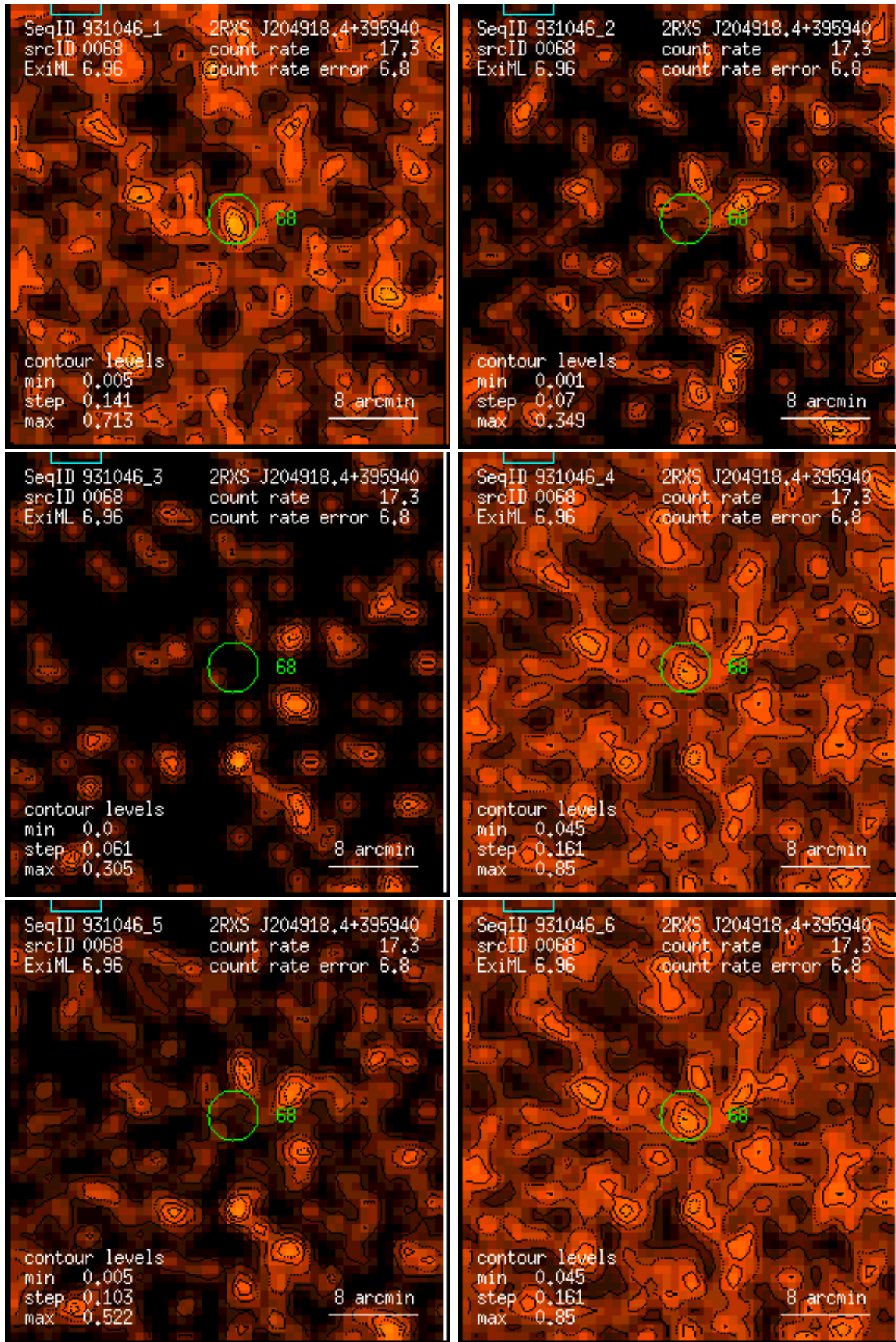
Figure 68: RASS 931046: detection 0068: band rate images, Gaussian filter: (1) PSPC channels 11 – 41, (2) 52 – 90, (3) 91 – 201, (4) 11 – 235, (5) 52 – 201, (6) 11 – 201. Broad band rates in counts/ks. Band rate contour levels in counts/ks/arcmin 2 .
