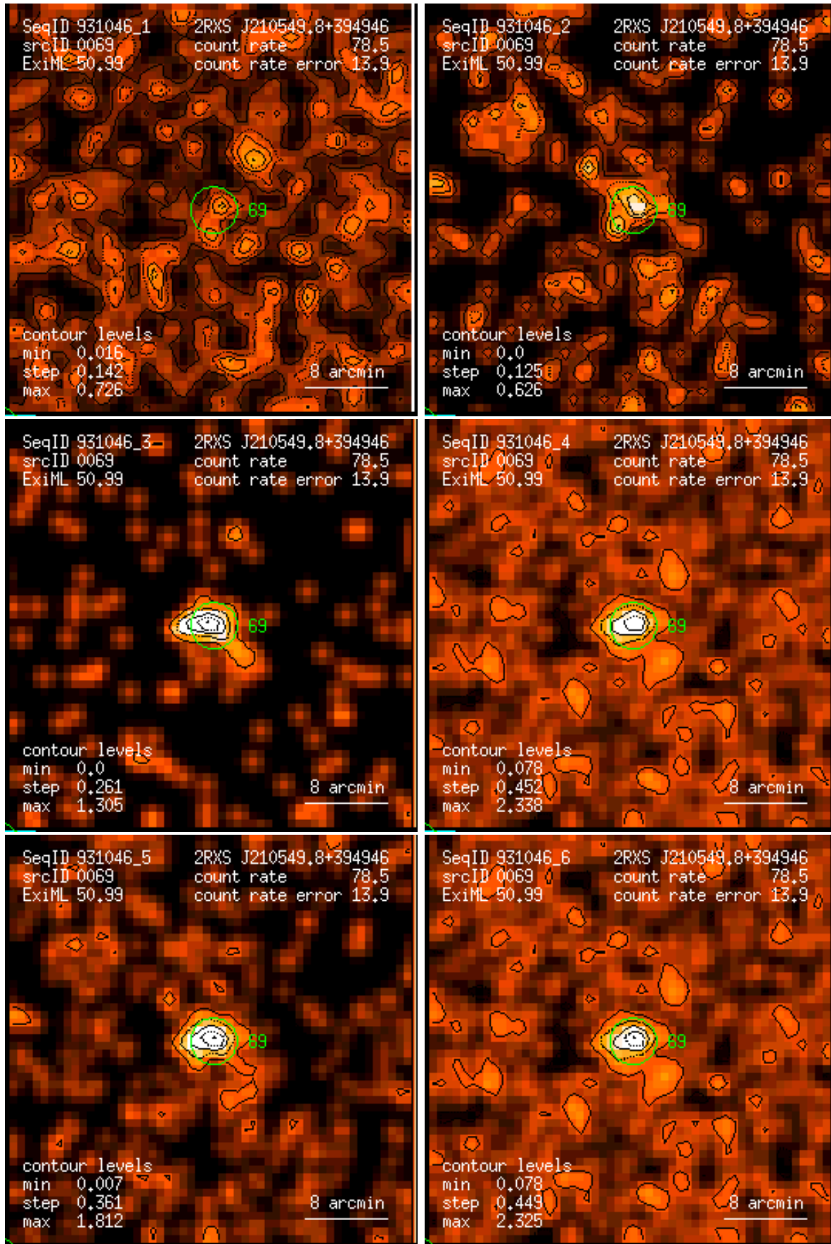
Figure 69: RASS 931046: detection 0069: band rate images, Gaussian filter: (1) PSPC channels 11 – 41, (2) 52 – 90, (3) 91 – 201, (4) 11 – 235, (5) 52 – 201, (6) 11 – 201. Broad band rates in counts/ks. Band rate contour levels in counts/ks/arcmin 2 .
