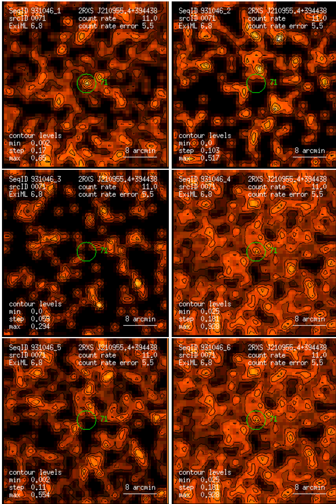
Figure 71: RASS 931046: detection 0071: band rate images, Gaussian filter: (1) PSPC channels 11 – 41, (2) 52 – 90, (3) 91 – 201, (4) 11 – 235, (5) 52 – 201, (6) 11 – 201. Broad band rates in counts/ks. Band rate contour levels in counts/ks/arcmin 2 .
