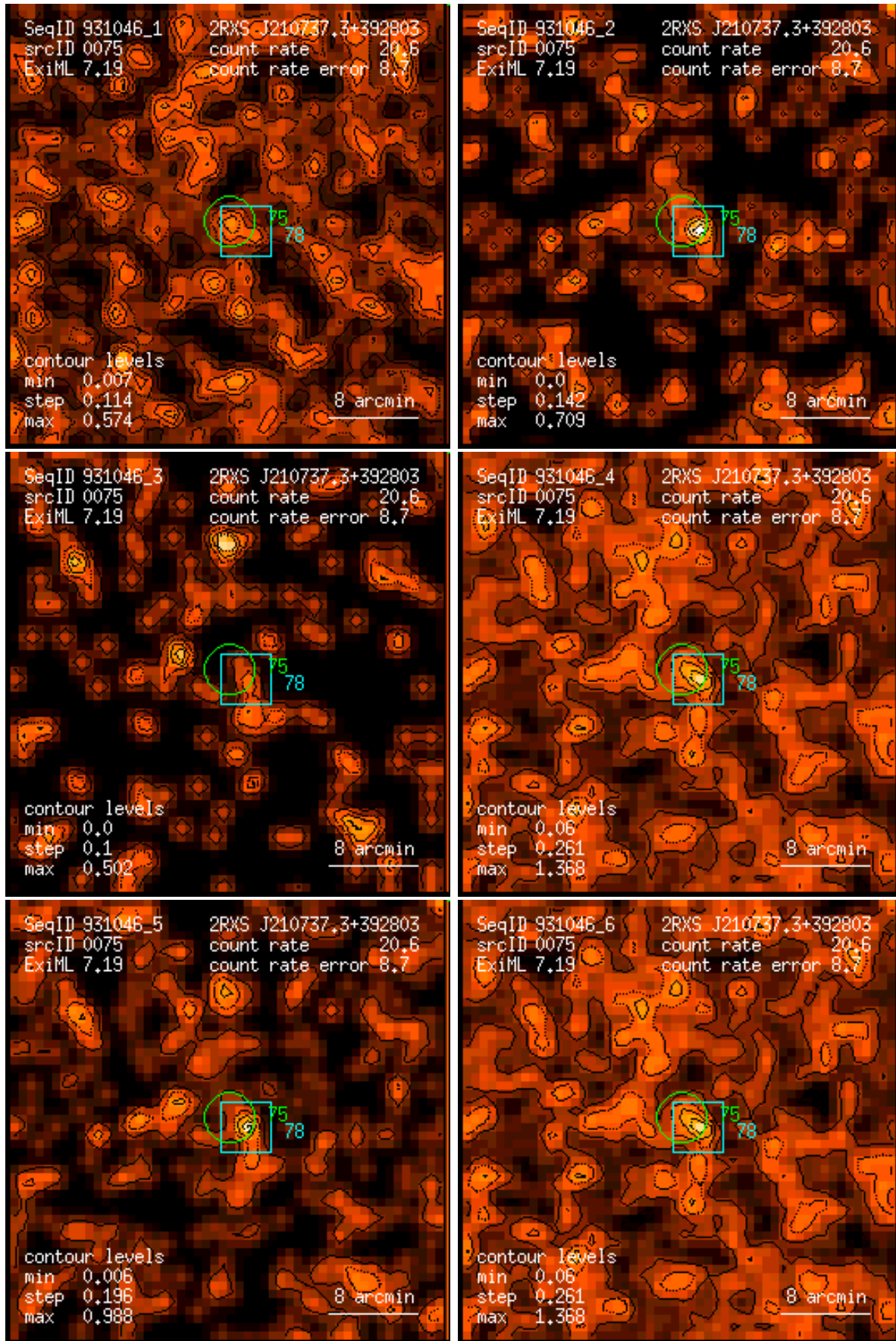
Figure 75: RASS 931046: detection 0075: band rate images, Gaussian filter: (1) PSPC channels 11 – 41, (2) 52 – 90, (3) 91 – 201, (4) 11 – 235, (5) 52 – 201, (6) 11 – 201. Broad band rates in counts/ks. Band rate contour levels in counts/ks/arcmin 2 .
