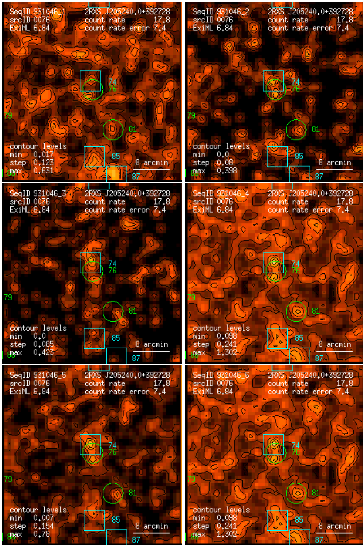
Figure 76: RASS 931046: detection 0076: band rate images, Gaussian filter: (1) PSPC channels 11 – 41, (2) 52 – 90, (3) 91 – 201, (4) 11 – 235, (5) 52 – 201, (6) 11 – 201. Broad band rates in counts/ks. Band rate contour levels in counts/ks/arcmin 2 .
