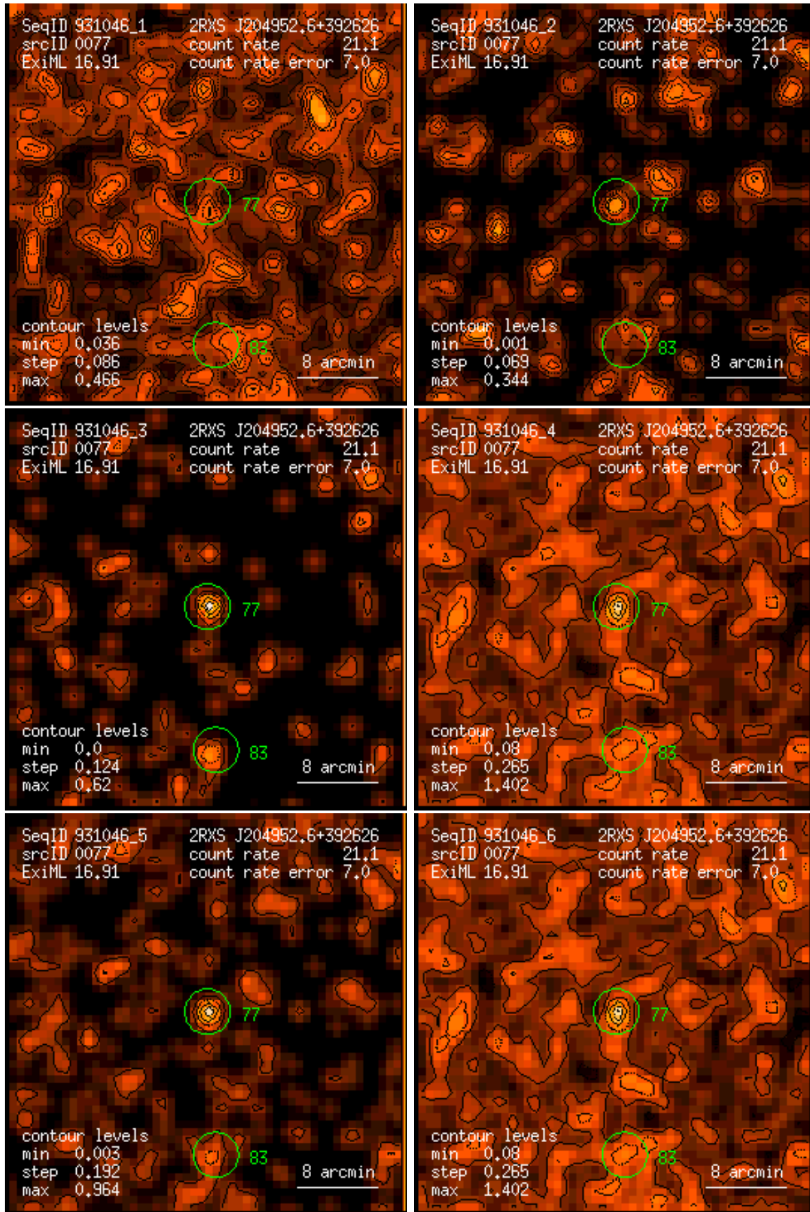
Figure 77: RASS 931046: detection 0077: band rate images, Gaussian filter: (1) PSPC channels 11 – 41, (2) 52 – 90, (3) 91 – 201, (4) 11 – 235, (5) 52 – 201, (6) 11 – 201. Broad band rates in counts/ks. Band rate contour levels in counts/ks/arcmin 2 .
