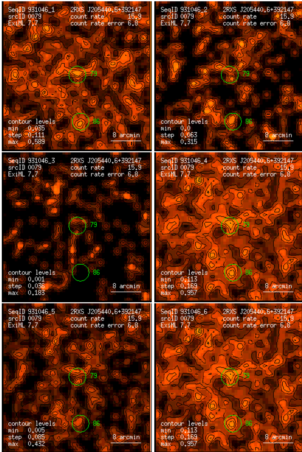
Figure 79: RASS 931046: detection 0079: band rate images, Gaussian filter: (1) PSPC channels 11 – 41, (2) 52 – 90, (3) 91 – 201, (4) 11 – 235, (5) 52 – 201, (6) 11 – 201. Broad band rates in counts/ks. Band rate contour levels in counts/ks/arcmin 2 .
