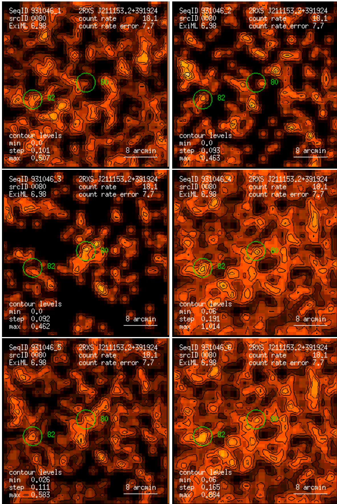
Figure 80: RASS 931046: detection 0080: band rate images, Gaussian filter: (1) PSPC channels 11 – 41, (2) 52 – 90, (3) 91 – 201, (4) 11 – 235, (5) 52 – 201, (6) 11 – 201. Broad band rates in counts/ks. Band rate contour levels in counts/ks/arcmin 2 .
