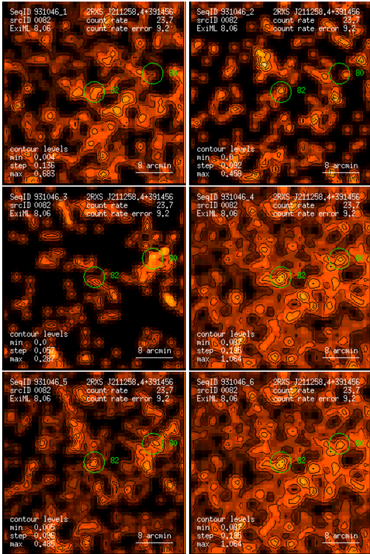
Figure 82: RASS 931046: detection 0082: band rate images, Gaussian filter: (1) PSPC channels 11 – 41, (2) 52 – 90, (3) 91 – 201, (4) 11 – 235, (5) 52 – 201, (6) 11 – 201. Broad band rates in counts/ks. Band rate contour levels in counts/ks/arcmin 2 .
