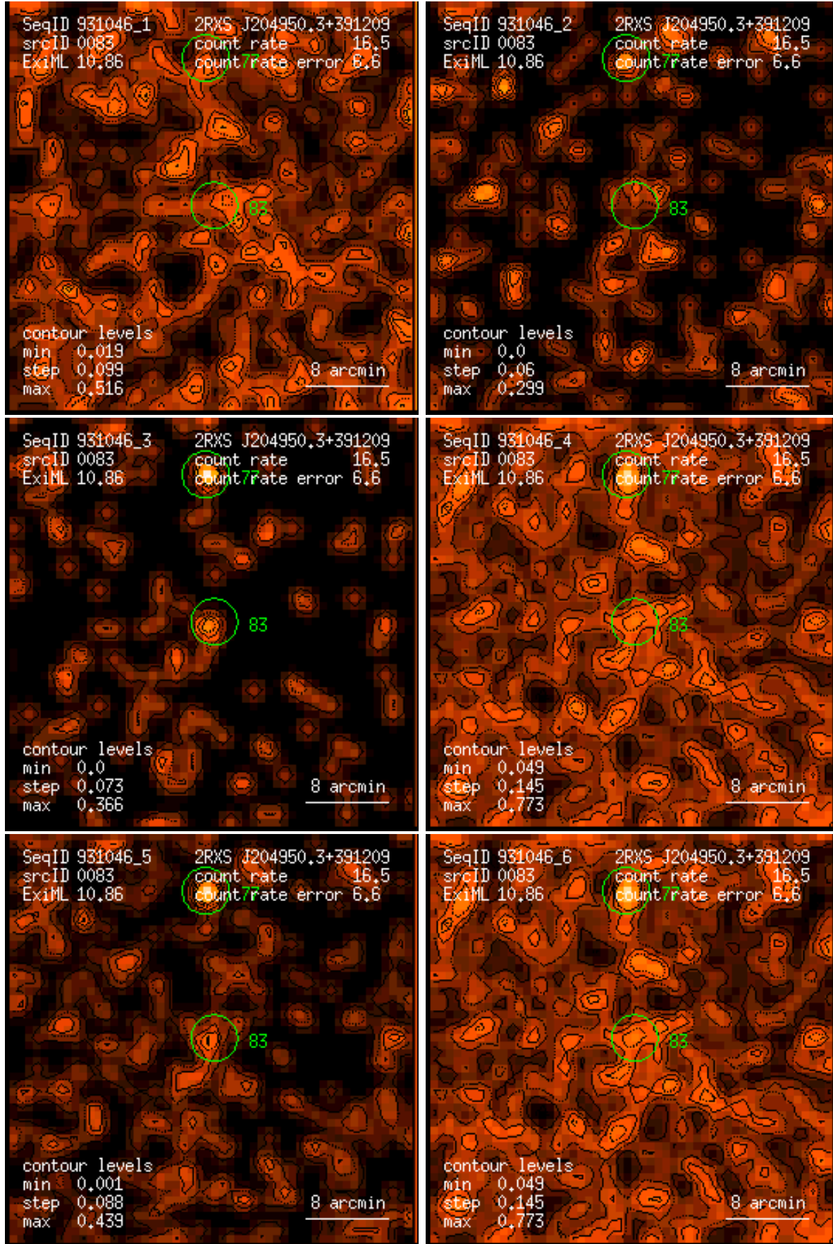
Figure 83: RASS 931046: detection 0083: band rate images, Gaussian filter: (1) PSPC channels 11 – 41, (2) 52 – 90, (3) 91 – 201, (4) 11 – 235, (5) 52 – 201, (6) 11 – 201. Broad band rates in counts/ks. Band rate contour levels in counts/ks/arcmin 2 .
