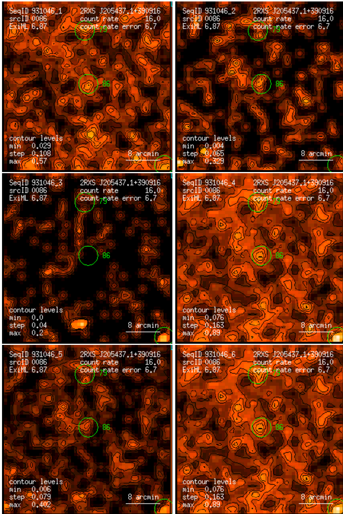
Figure 86: RASS 931046: detection 0086: band rate images, Gaussian filter: (1) PSPC channels 11 – 41, (2) 52 – 90, (3) 91 – 201, (4) 11 – 235, (5) 52 – 201, (6) 11 – 201. Broad band rates in counts/ks. Band rate contour levels in counts/ks/arcmin 2 .
