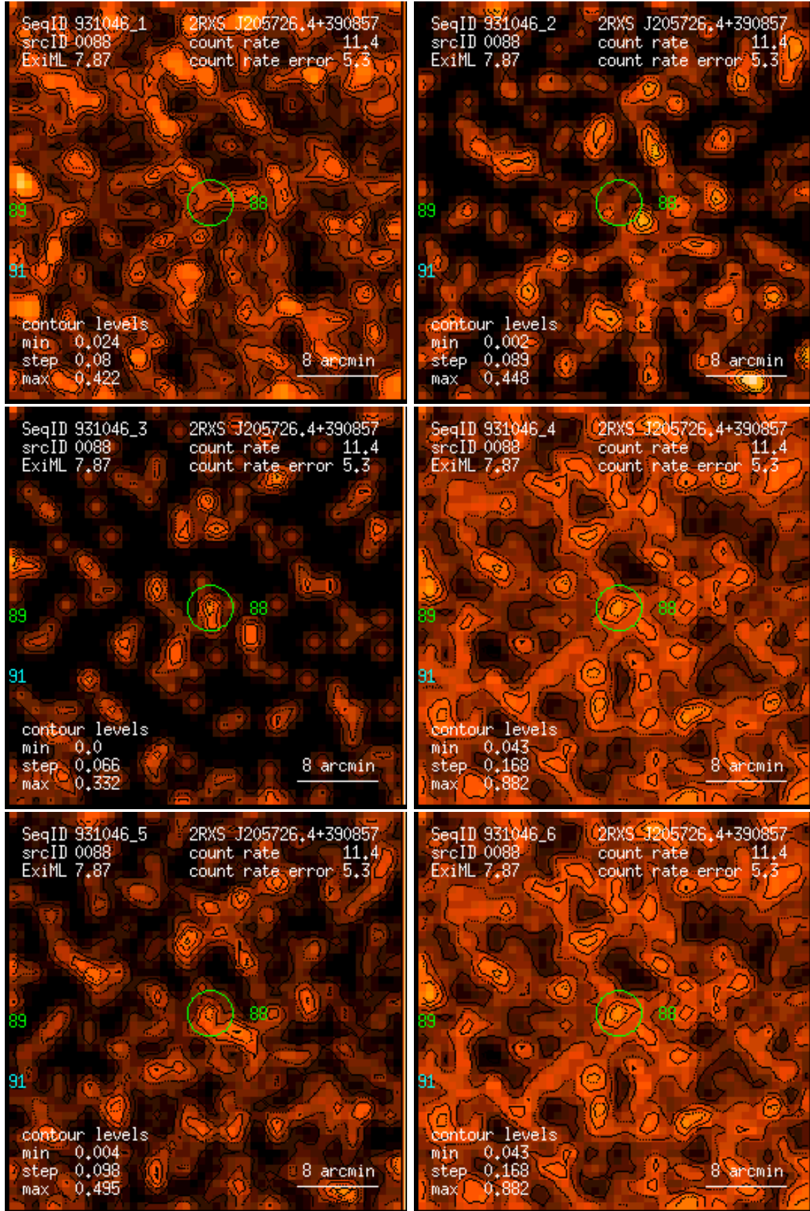
Figure 88: RASS 931046: detection 0088: band rate images, Gaussian filter: (1) PSPC channels 11 – 41, (2) 52 – 90, (3) 91 – 201, (4) 11 – 235, (5) 52 – 201, (6) 11 – 201. Broad band rates in counts/ks. Band rate contour levels in counts/ks/arcmin 2 .
