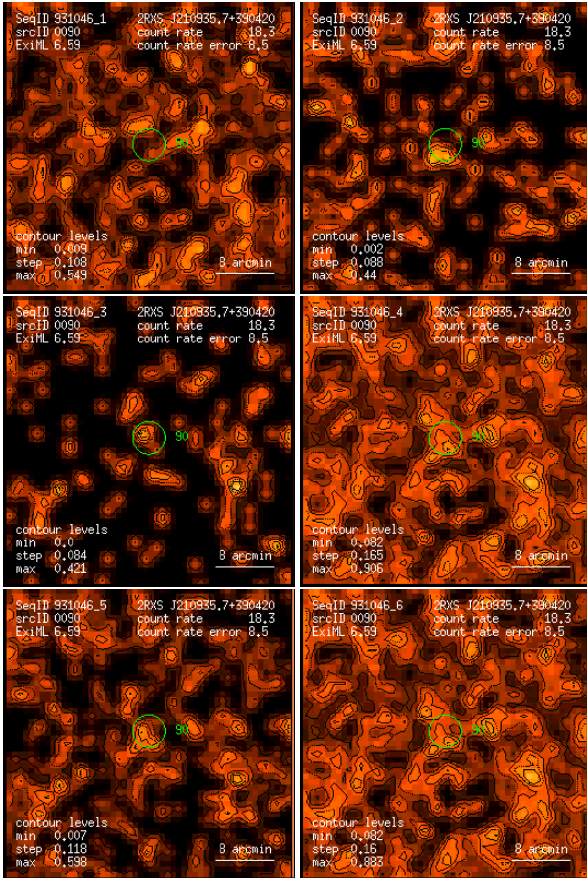
Figure 90: RASS 931046: detection 0090: band rate images, Gaussian filter: (1) PSPC channels 11 – 41, (2) 52 – 90, (3) 91 – 201, (4) 11 – 235, (5) 52 – 201, (6) 11 – 201. Broad band rates in counts/ks. Band rate contour levels in counts/ks/arcmin 2 .
