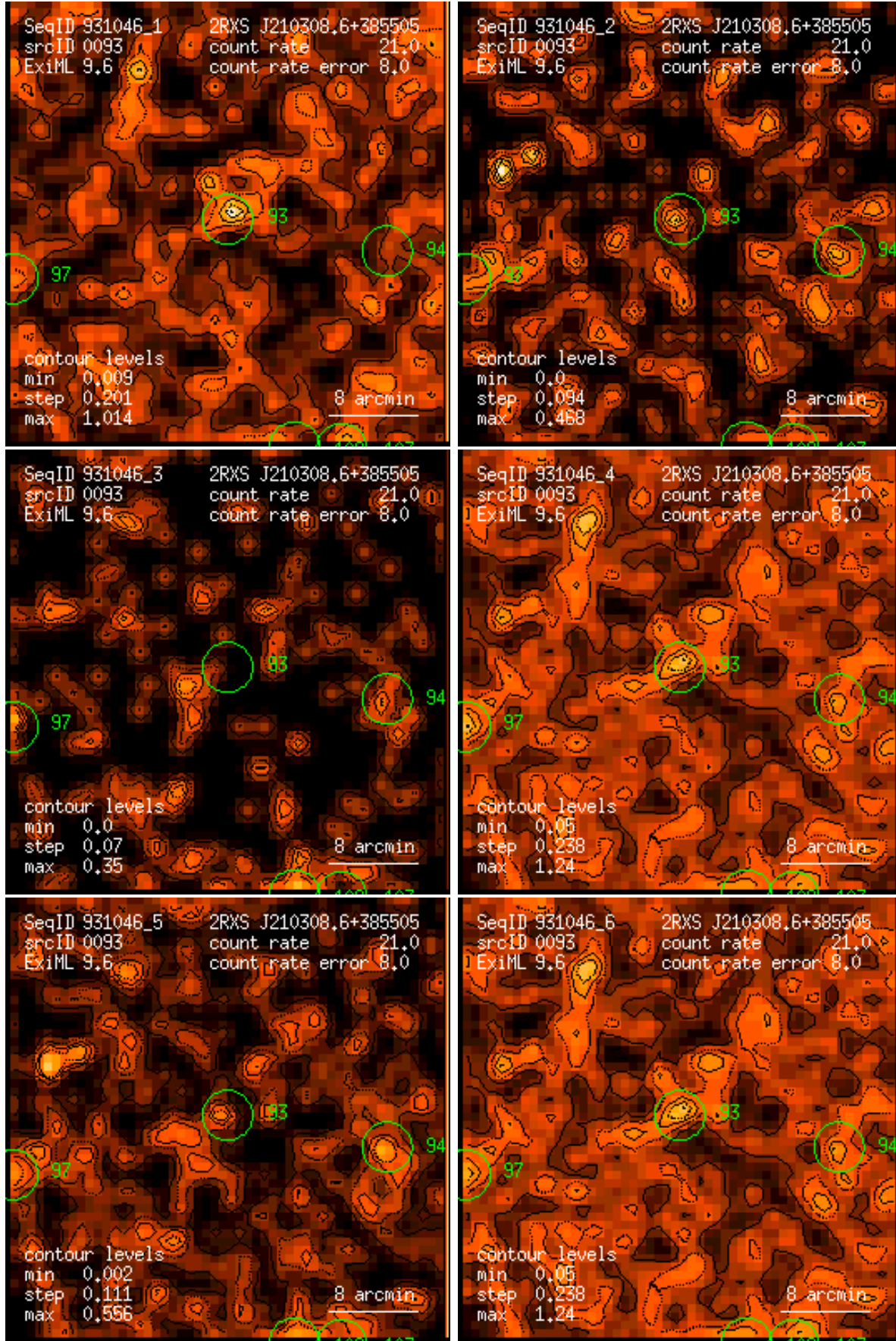
Figure 93: RASS 931046: detection 0093: band rate images, Gaussian filter: (1) PSPC channels 11 – 41, (2) 52 – 90, (3) 91 – 201, (4) 11 – 235, (5) 52 – 201, (6) 11 – 201. Broad band rates in counts/ks. Band rate contour levels in counts/ks/arcmin 2 .
