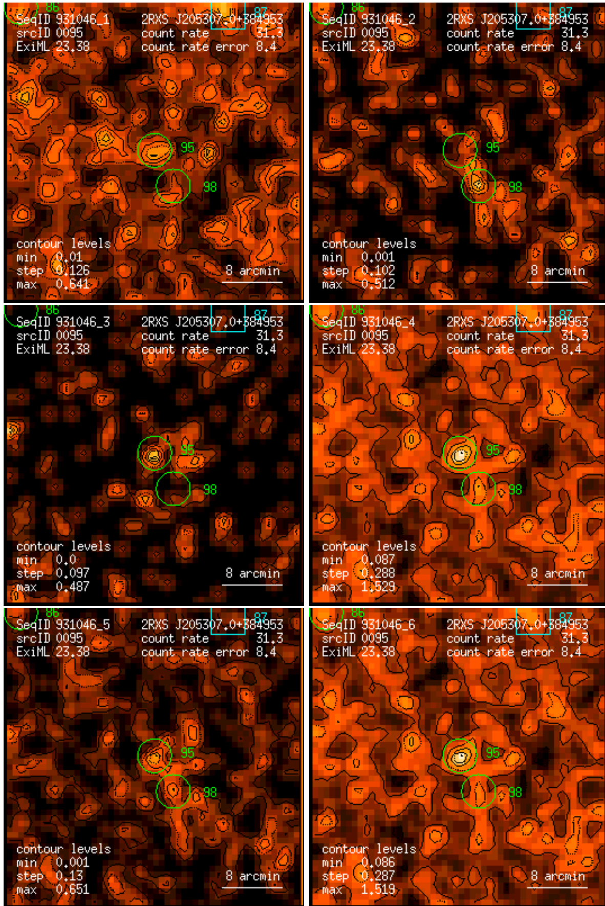
Figure 95: RASS 931046: detection 0095: band rate images, Gaussian filter: (1) PSPC channels 11 – 41, (2) 52 – 90, (3) 91 – 201, (4) 11 – 235, (5) 52 – 201, (6) 11 – 201. Broad band rates in counts/ks. Band rate contour levels in counts/ks/arcmin 2 .
