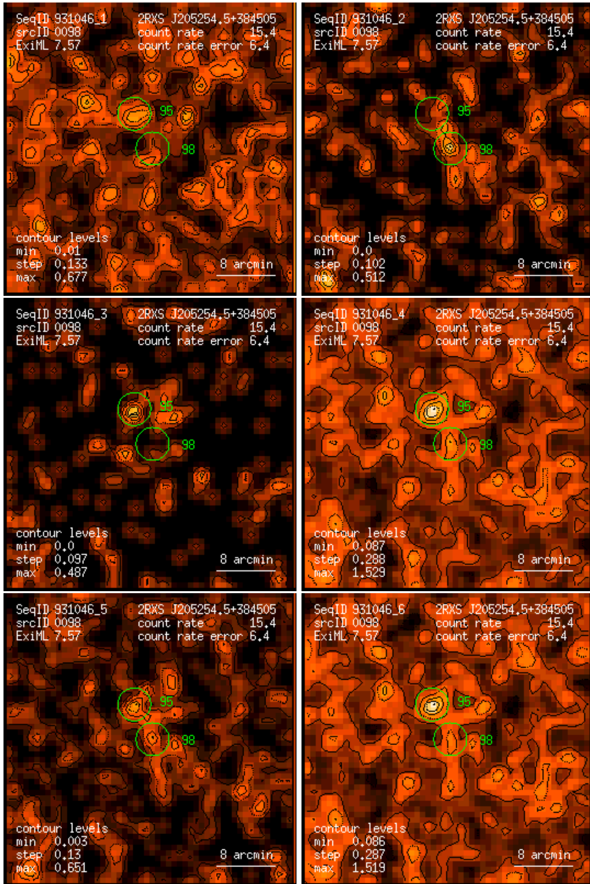
Figure 98: RASS 931046: detection 0098: band rate images, Gaussian filter: (1) PSPC channels 11 – 41, (2) 52 – 90, (3) 91 – 201, (4) 11 – 235, (5) 52 – 201, (6) 11 – 201. Broad band rates in counts/ks. Band rate contour levels in counts/ks/arcmin 2 .
