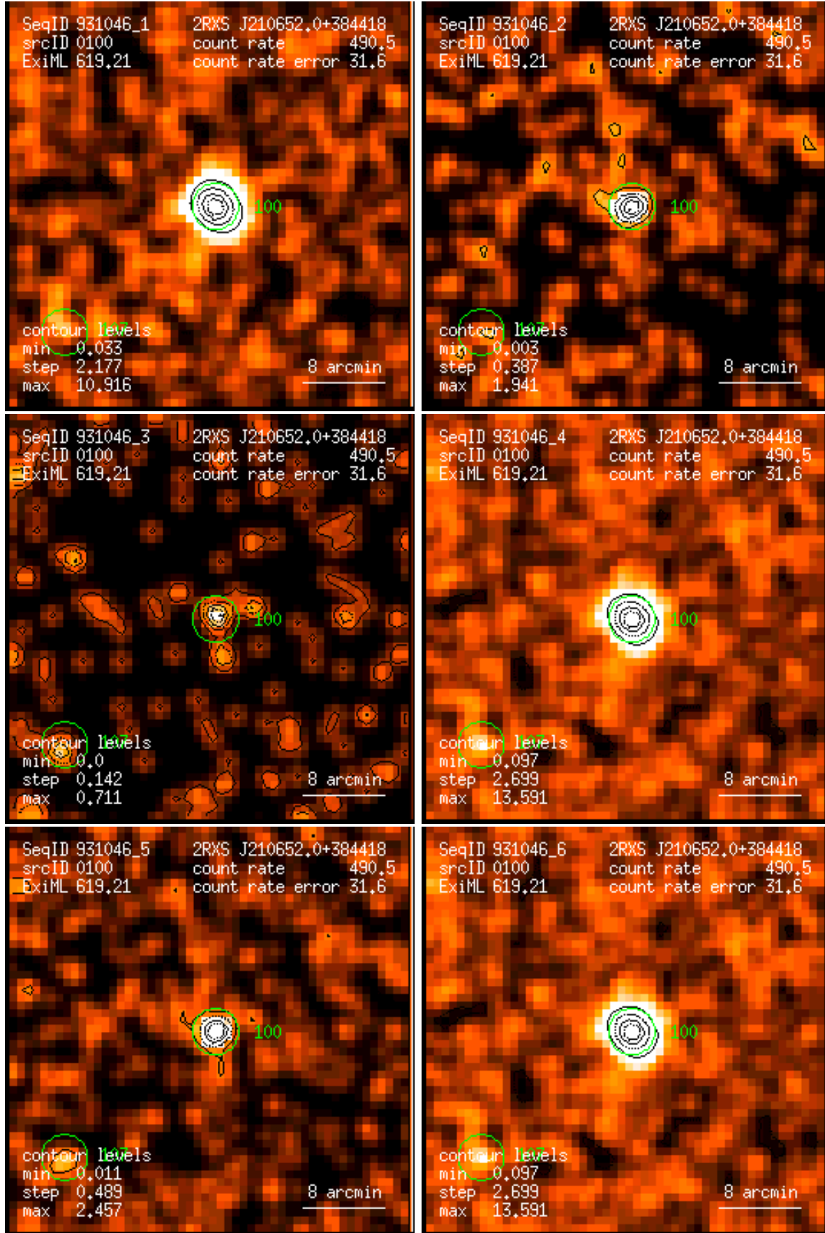
Figure 100: RASS 931046: detection 0100: band rate images, Gaussian filter: (1) PSPC channels 11 – 41, (2) 52 – 90, (3) 91 – 201, (4) 11 – 235, (5) 52 – 201, (6) 11 – 201. Broad band rates in counts/ks. Band rate contour levels in counts/ks/arcmin 2 .
