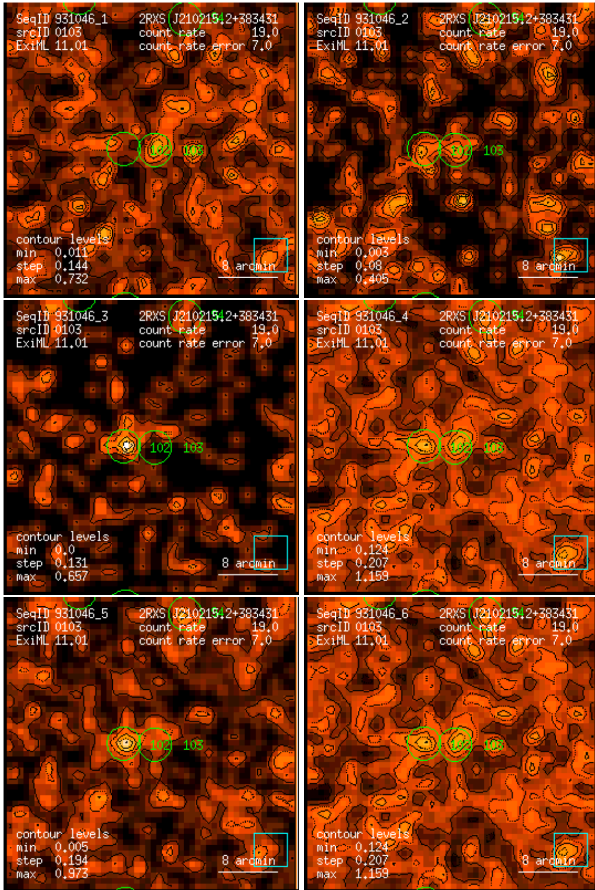
Figure 103: RASS 931046: detection 0103: band rate images, Gaussian filter: (1) PSPC channels 11 – 41, (2) 52 – 90, (3) 91 – 201, (4) 11 – 235, (5) 52 – 201, (6) 11 – 201. Broad band rates in counts/ks. Band rate contour levels in counts/ks/arcmin 2 .
