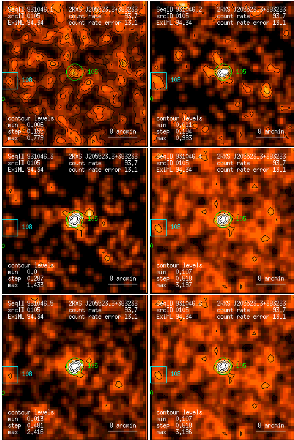
Figure 105: RASS 931046: detection 0105: band rate images, Gaussian filter: (1) PSPC channels 11 – 41, (2) 52 – 90, (3) 91 – 201, (4) 11 – 235, (5) 52 – 201, (6) 11 – 201. Broad band rates in counts/ks. Band rate contour levels in counts/ks/arcmin 2 .
