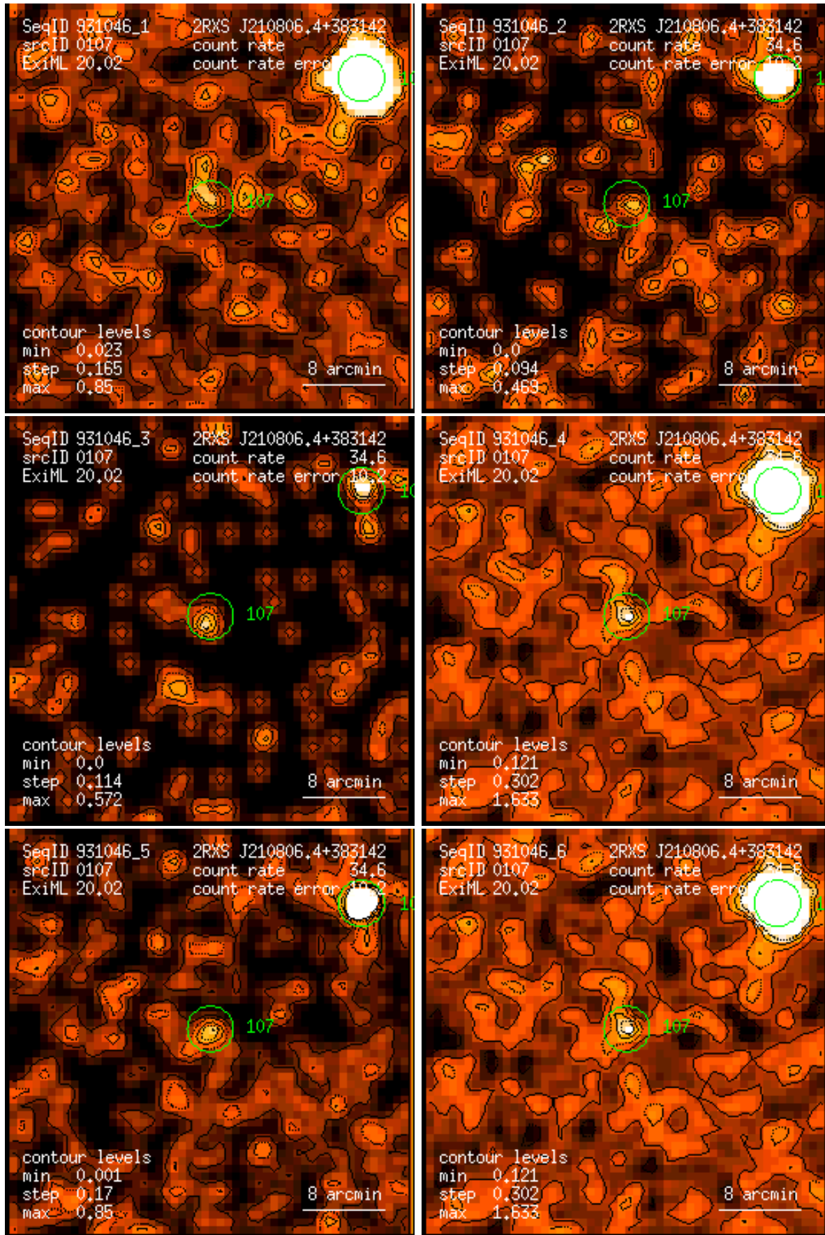
Figure 107: RASS 931046: detection 0107: band rate images, Gaussian filter: (1) PSPC channels 11 – 41, (2) 52 – 90, (3) 91 – 201, (4) 11 – 235, (5) 52 – 201, (6) 11 – 201. Broad band rates in counts/ks. Band rate contour levels in counts/ks/arcmin 2 .
