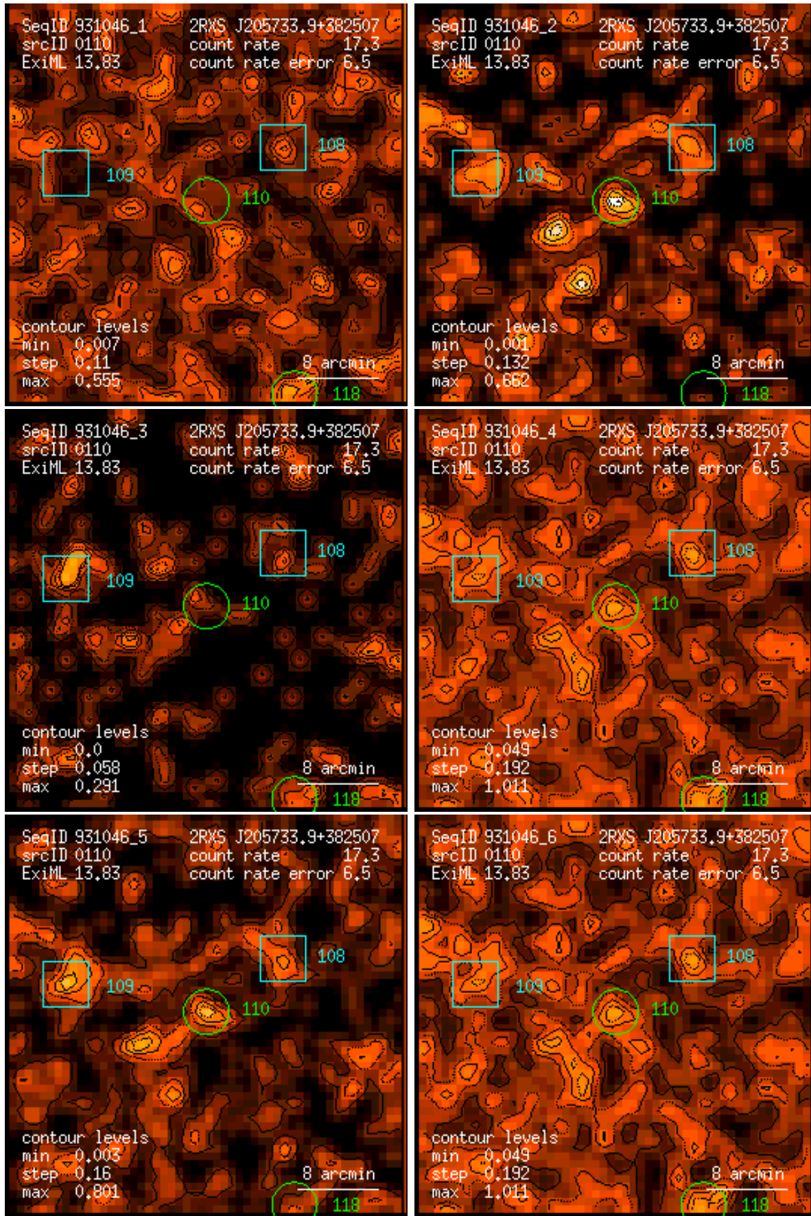
Figure 110: RASS 931046: detection 0110: band rate images, Gaussian filter: (1) PSPC channels 11 – 41, (2) 52 – 90, (3) 91 – 201, (4) 11 – 235, (5) 52 – 201, (6) 11 – 201. Broad band rates in counts/ks. Band rate contour levels in counts/ks/arcmin 2 .
