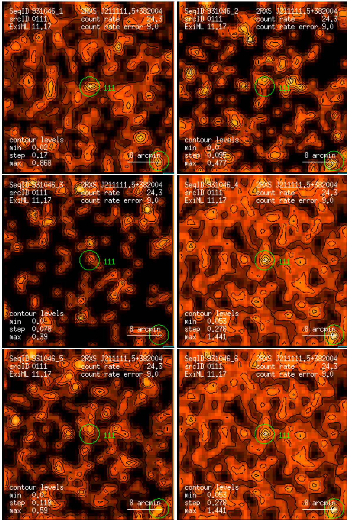
Figure 111: RASS 931046: detection 0111: band rate images, Gaussian filter: (1) PSPC channels 11 – 41, (2) 52 – 90, (3) 91 – 201, (4) 11 – 235, (5) 52 – 201, (6) 11 – 201. Broad band rates in counts/ks. Band rate contour levels in counts/ks/arcmin 2 .
