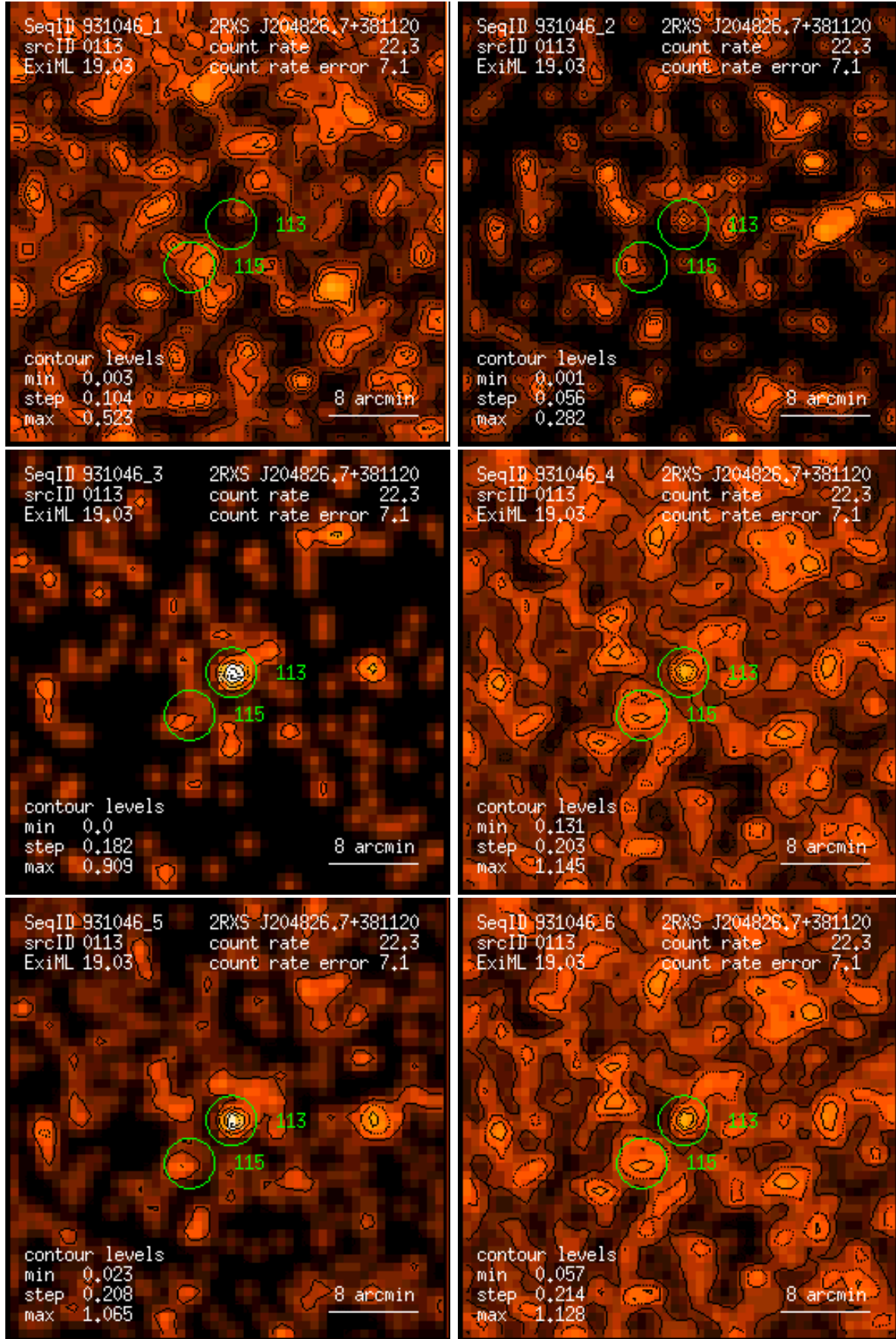
Figure 113: RASS 931046: detection 0113: band rate images, Gaussian filter: (1) PSPC channels 11 – 41, (2) 52 – 90, (3) 91 – 201, (4) 11 – 235, (5) 52 – 201, (6) 11 – 201. Broad band rates in counts/ks. Band rate contour levels in counts/ks/arcmin 2 .
