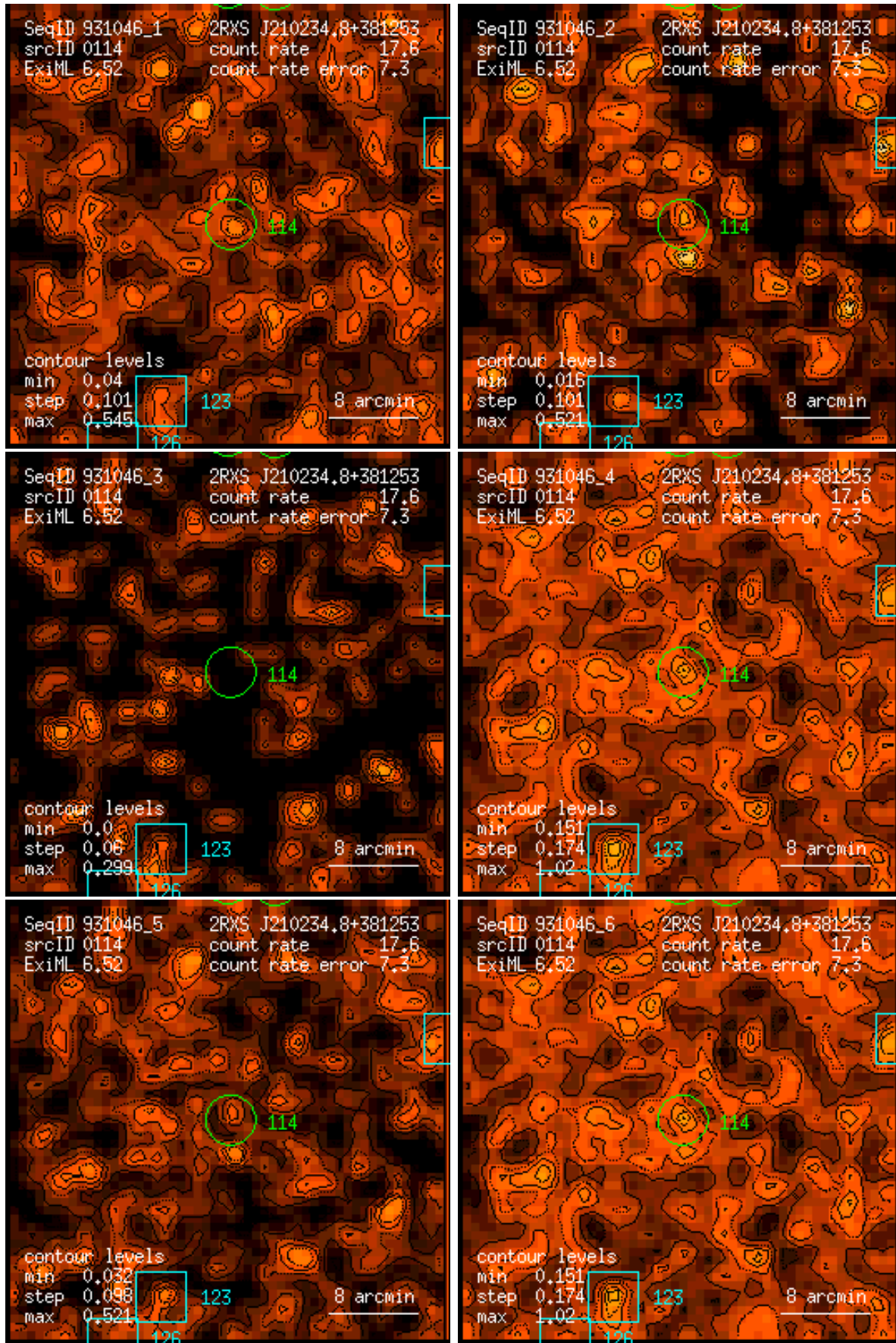
Figure 114: RASS 931046: detection 0114: band rate images, Gaussian filter: (1) PSPC channels 11 – 41, (2) 52 – 90, (3) 91 – 201, (4) 11 – 235, (5) 52 – 201, (6) 11 – 201. Broad band rates in counts/ks. Band rate contour levels in counts/ks/arcmin 2 .
