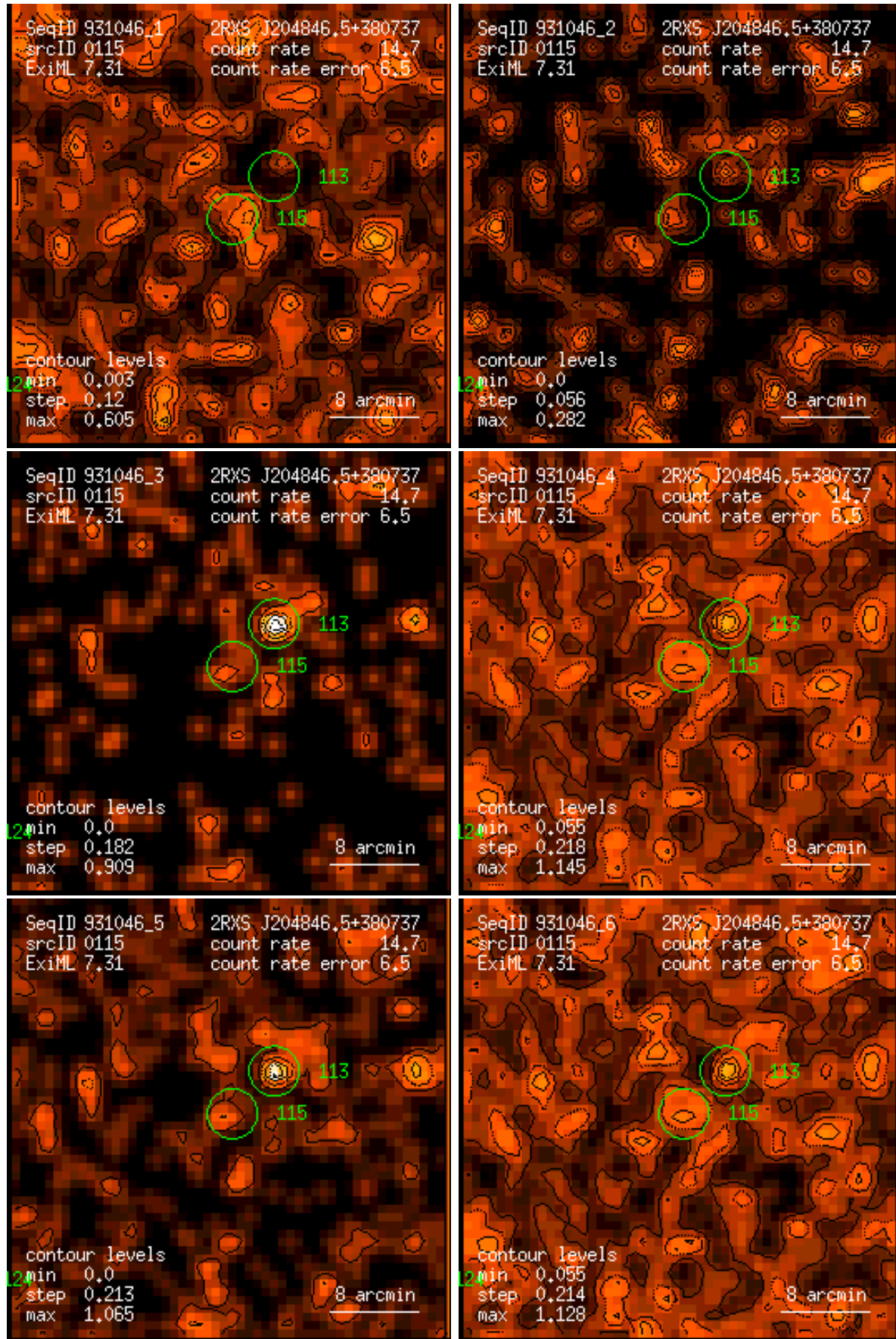
Figure 115: RASS 931046: detection 0115: band rate images, Gaussian filter: (1) PSPC channels 11 – 41, (2) 52 – 90, (3) 91 – 201, (4) 11 – 235, (5) 52 – 201, (6) 11 – 201. Broad band rates in counts/ks. Band rate contour levels in counts/ks/arcmin 2 .
