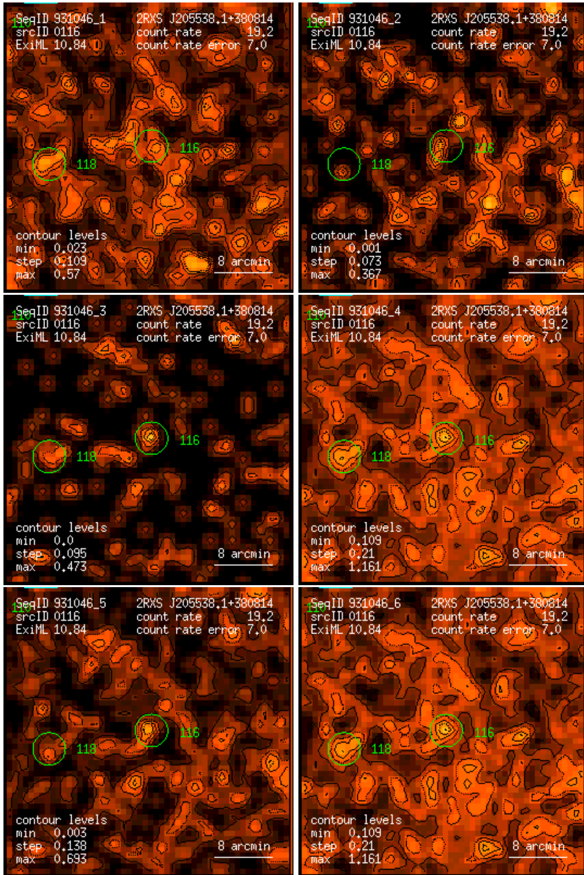
Figure 116: RASS 931046: detection 0116: band rate images, Gaussian filter: (1) PSPC channels 11 – 41, (2) 52 – 90, (3) 91 – 201, (4) 11 – 235, (5) 52 – 201, (6) 11 – 201. Broad band rates in counts/ks. Band rate contour levels in counts/ks/arcmin 2 .
