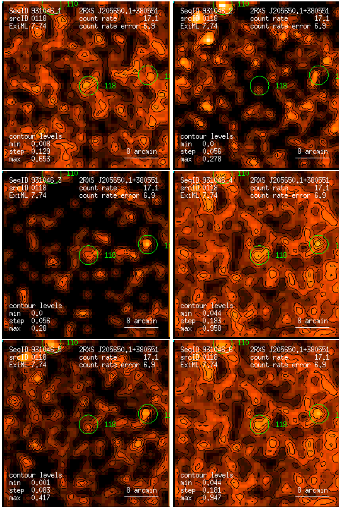
Figure 118: RASS 931046: detection 0118: band rate images, Gaussian filter: (1) PSPC channels 11 – 41, (2) 52 – 90, (3) 91 – 201, (4) 11 – 235, (5) 52 – 201, (6) 11 – 201. Broad band rates in counts/ks. Band rate contour levels in counts/ks/arcmin 2 .
