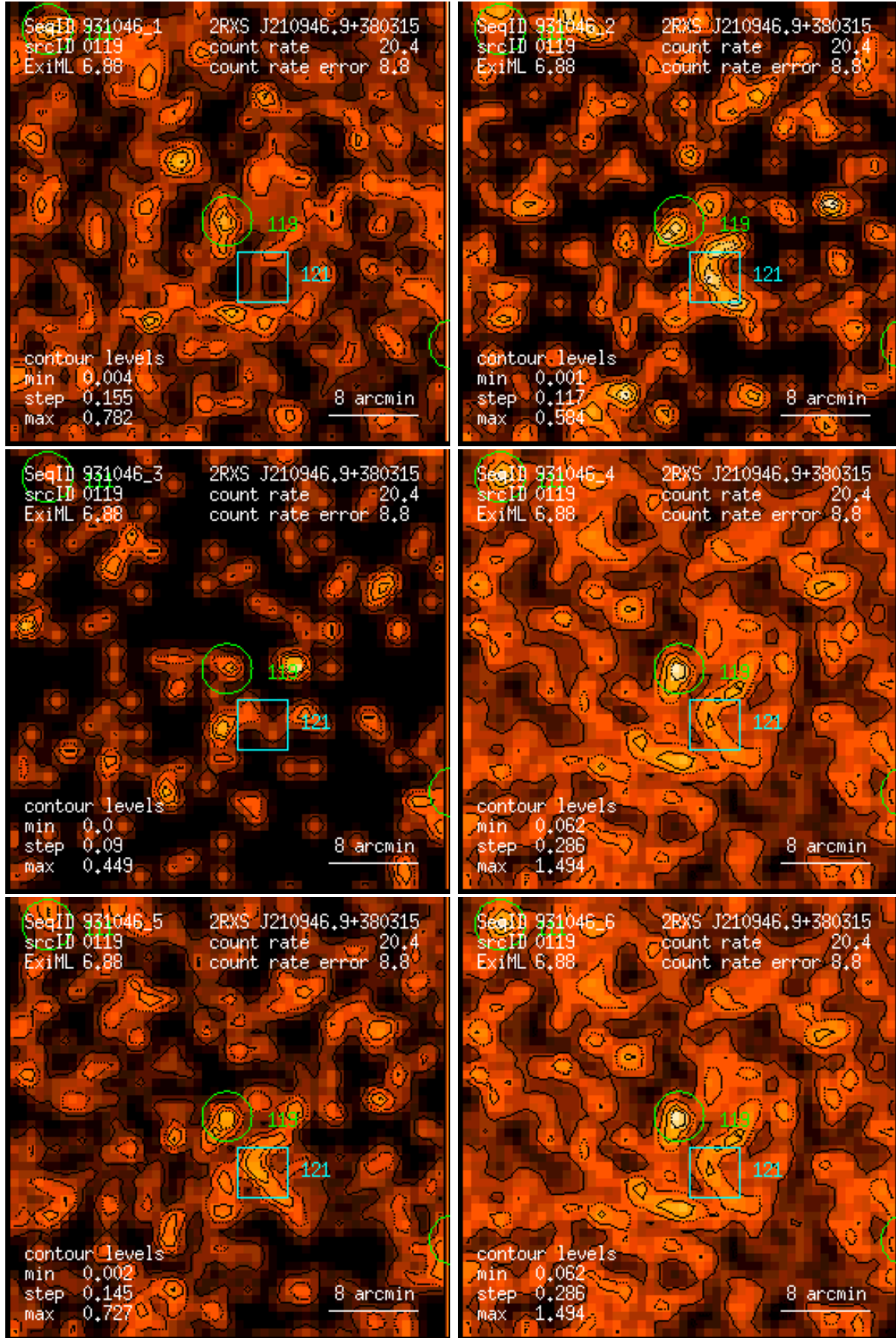
Figure 119: RASS 931046: detection 0119: band rate images, Gaussian filter: (1) PSPC channels 11 – 41, (2) 52 – 90, (3) 91 – 201, (4) 11 – 235, (5) 52 – 201, (6) 11 – 201. Broad band rates in counts/ks. Band rate contour levels in counts/ks/arcmin 2 .
