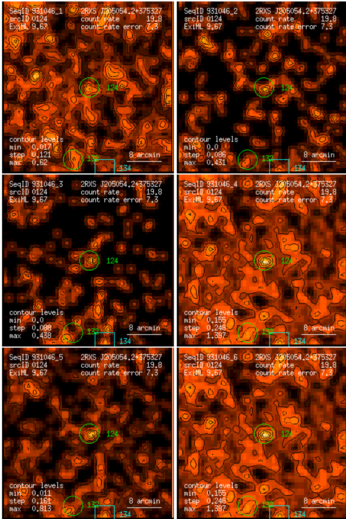
Figure 124: RASS 931046: detection 0124: band rate images, Gaussian filter: (1) PSPC channels 11 – 41, (2) 52 – 90, (3) 91 – 201, (4) 11 – 235, (5) 52 – 201, (6) 11 – 201. Broad band rates in counts/ks. Band rate contour levels in counts/ks/arcmin 2 .
