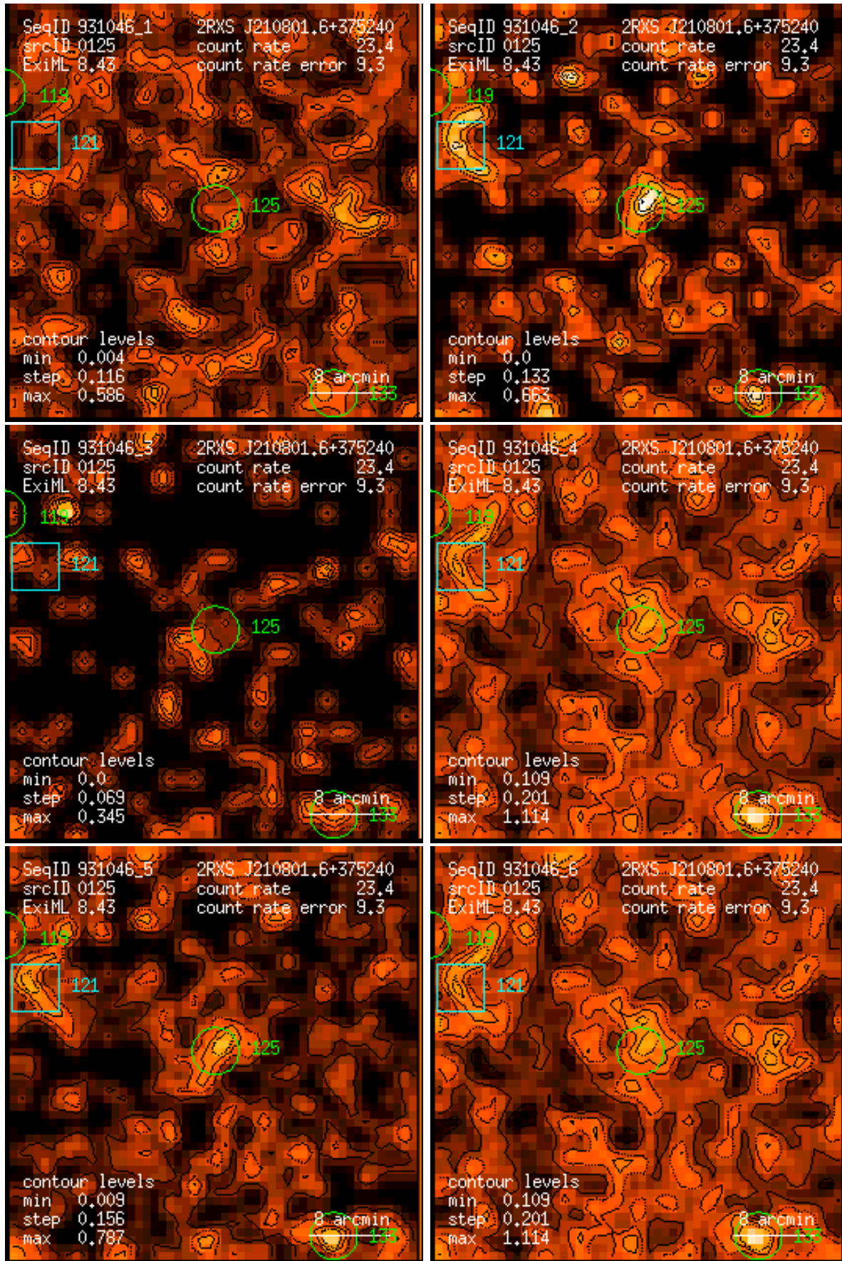
Figure 125: RASS 931046: detection 0125: band rate images, Gaussian filter: (1) PSPC channels 11 – 41, (2) 52 – 90, (3) 91 – 201, (4) 11 – 235, (5) 52 – 201, (6) 11 – 201. Broad band rates in counts/ks. Band rate contour levels in counts/ks/arcmin 2 .
