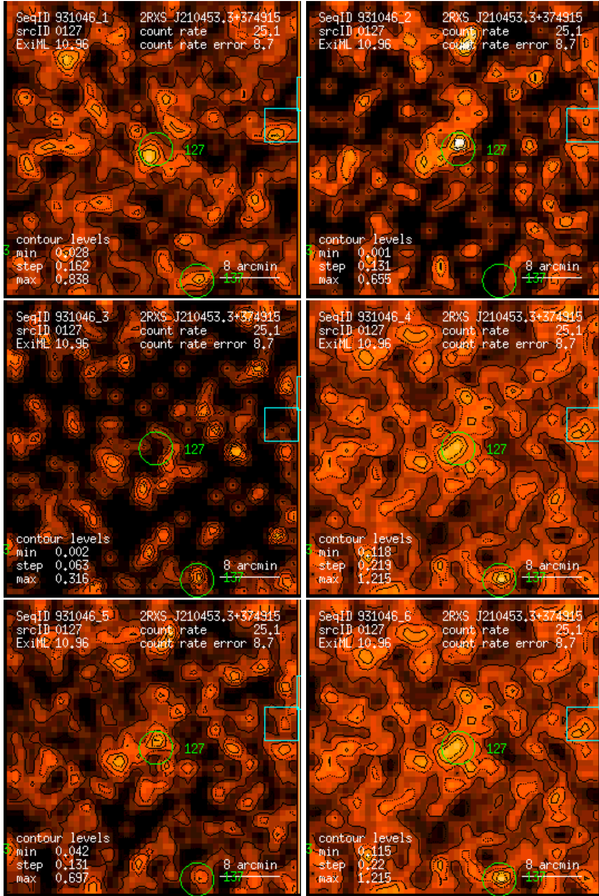
Figure 127: RASS 931046: detection 0127: band rate images, Gaussian filter: (1) PSPC channels 11 – 41, (2) 52 – 90, (3) 91 – 201, (4) 11 – 235, (5) 52 – 201, (6) 11 – 201. Broad band rates in counts/ks. Band rate contour levels in counts/ks/arcmin 2 .
